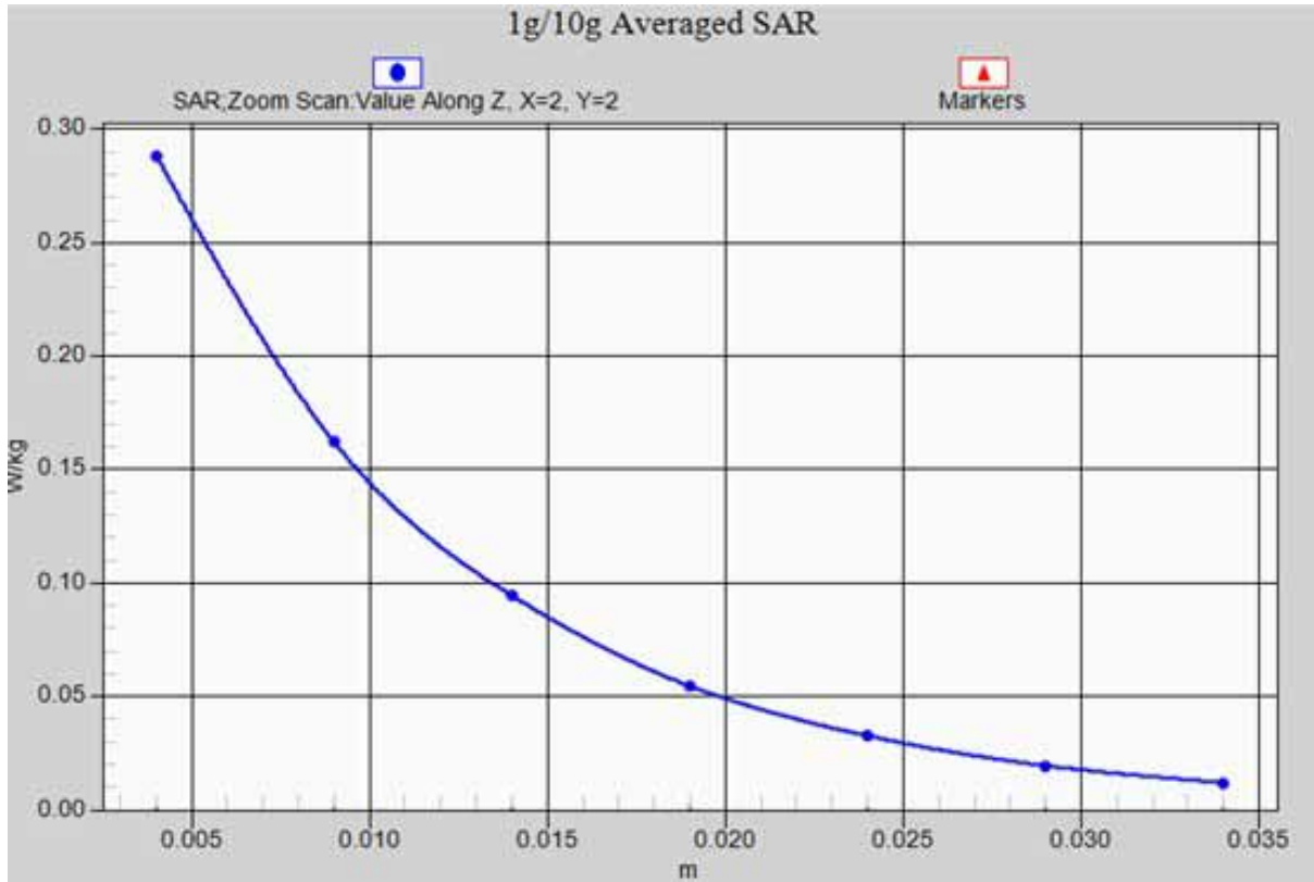
(SISO mode)Back side Low without external antenna_ z-axis scan
