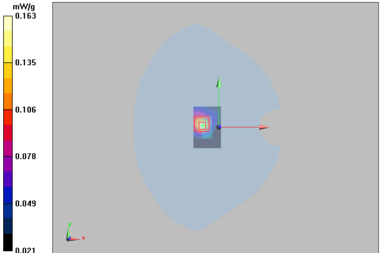
Figure 9 802.11b with IBM T61 Test Position 1 Channel 1
