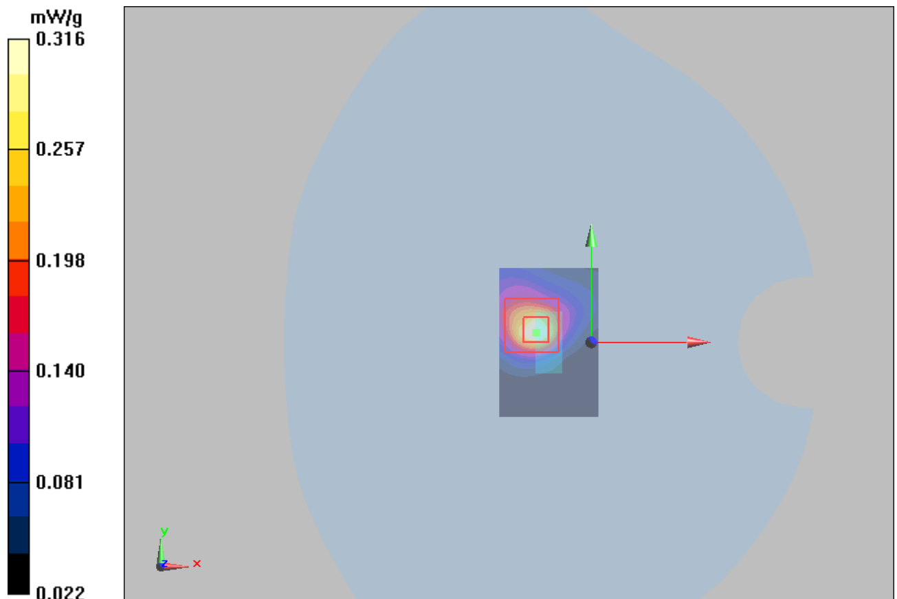
Figure 7 802.11b with IBM T61 Test Position 1 Channel 11
