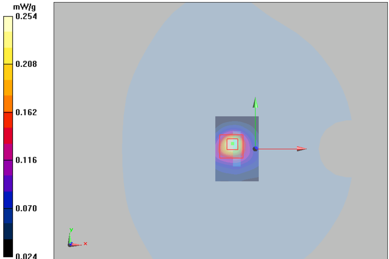
Figure 13 802.11b with IBM T61 Test Position 5 Channel 6
