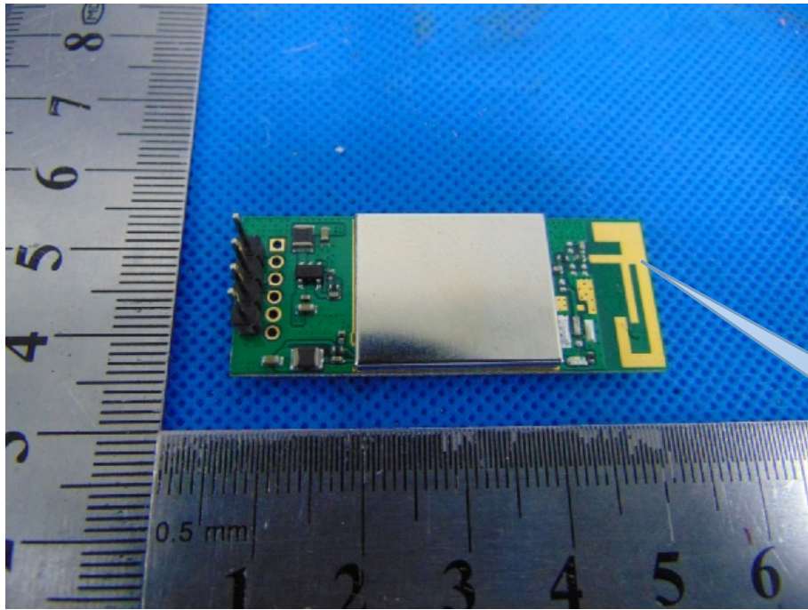
WiFi Antenna location
