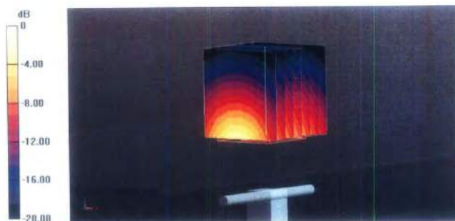
0 dB = 20.6 W/kg = 13.14 dBW/kg
