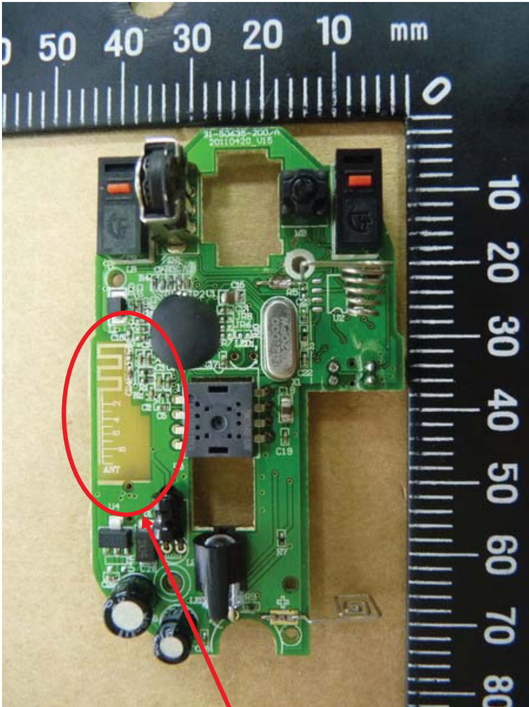
PCB Antenna
