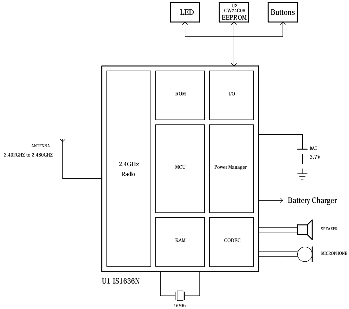
Block Diagram
