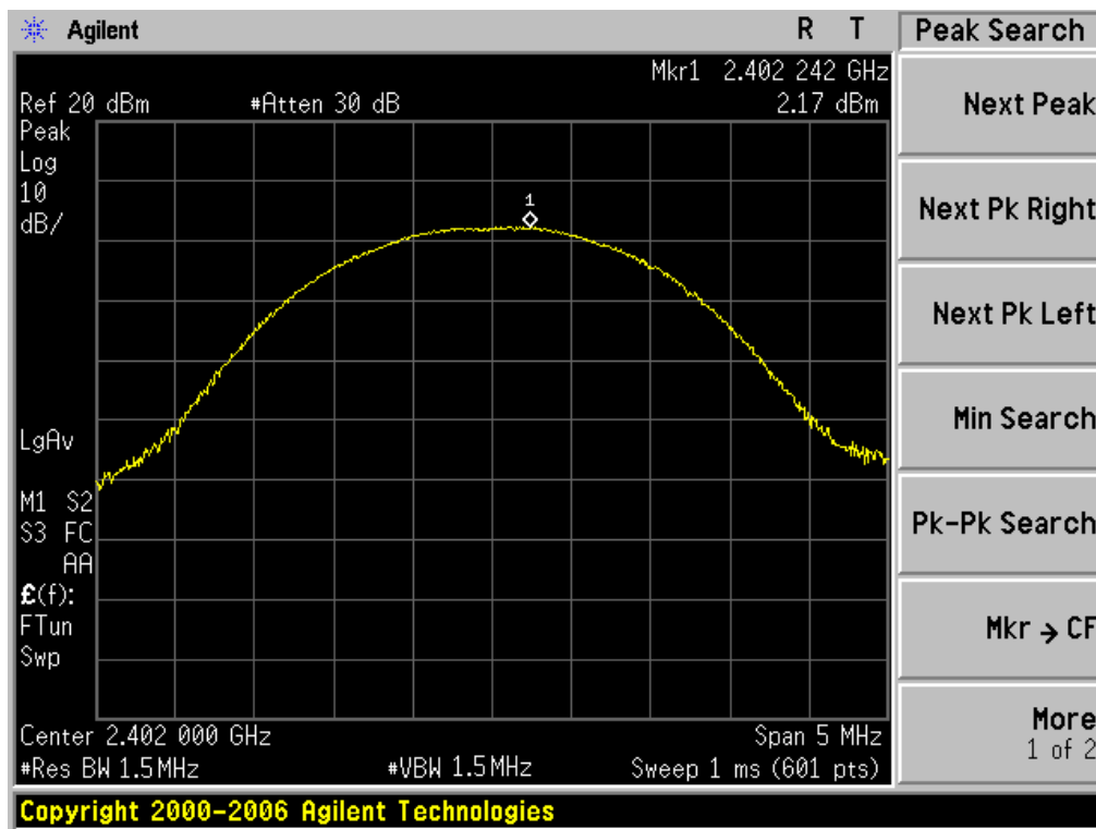
TEST PLOT OF PEAK POWER FOR LOW CHANNEL
