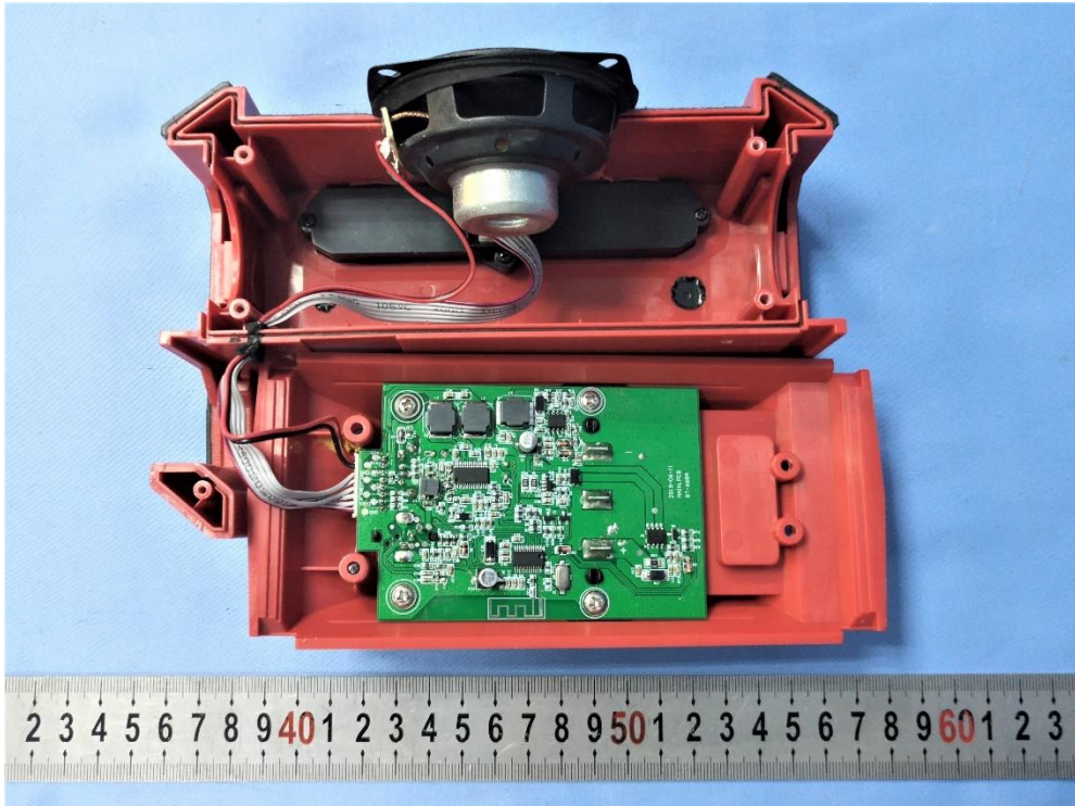
Internal Photo
