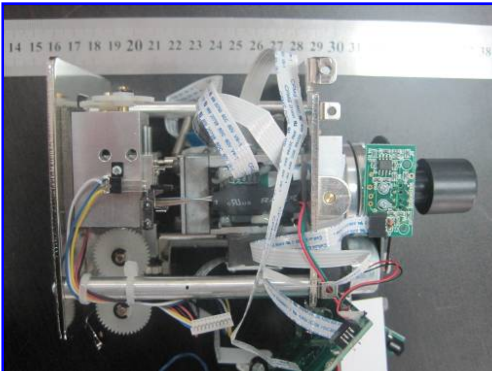
Rear View of Rotary Part
