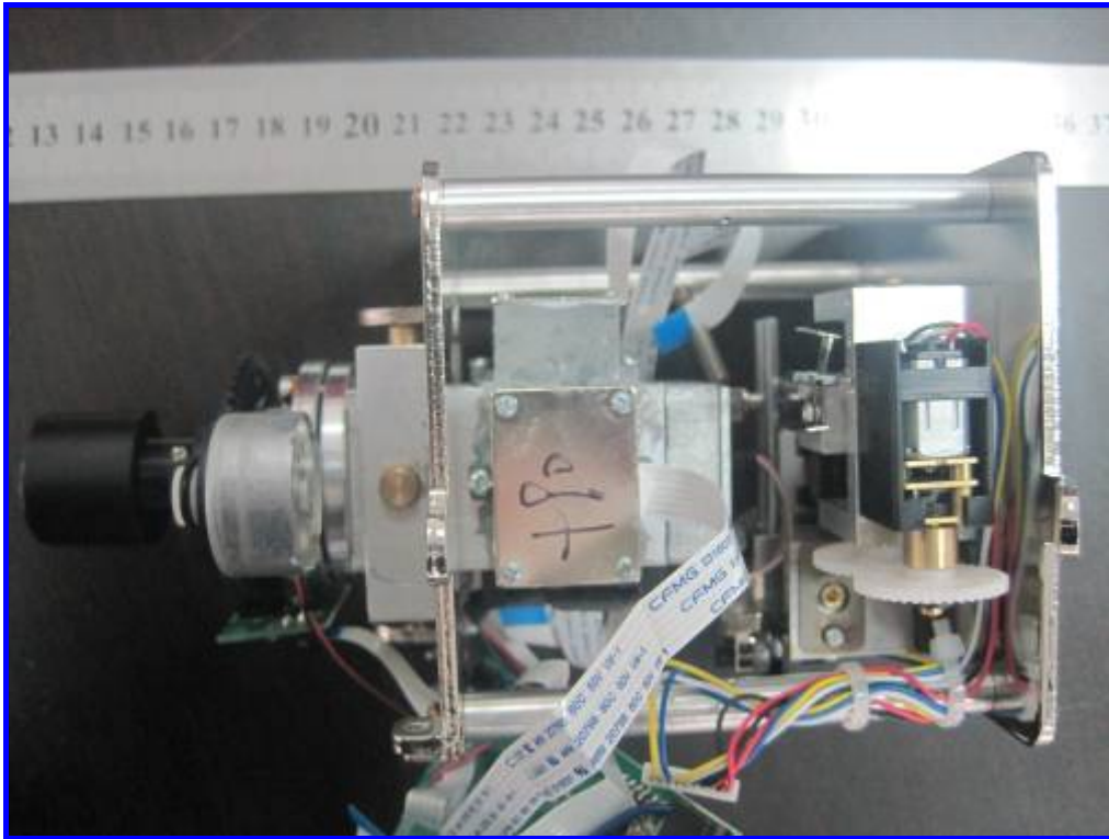
Left View of Rotary Part
