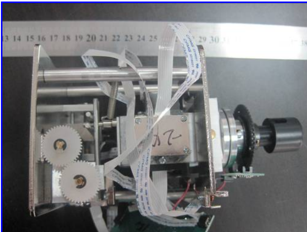
Right View of Rotary Part
