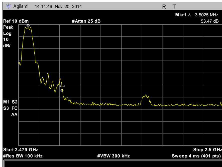
Plot 35. Conducted Band Edge, High Channel
