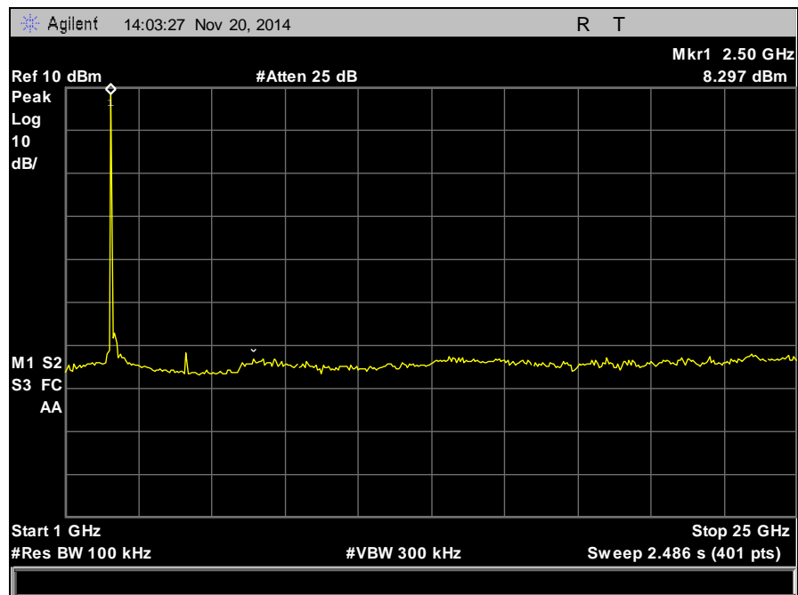
Plot 33. Conducted Spurious Emissions, High Channel, 1 GHz – 25 GHz
