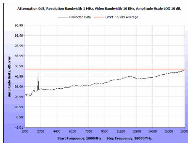
Plot 16. Radiated Spurious Emissions, Low Channel, 1 GHz – 18 GHz, Average
