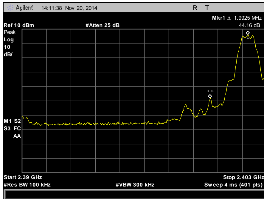
Plot 34. Conducted Band Edge, Low Channel
