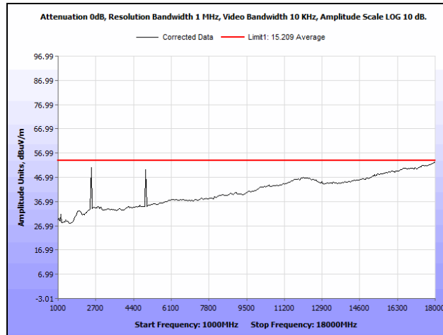
Plot 22. Radiated Spurious Emissions, High Channel, 1 GHz – 18 GHz, Average
