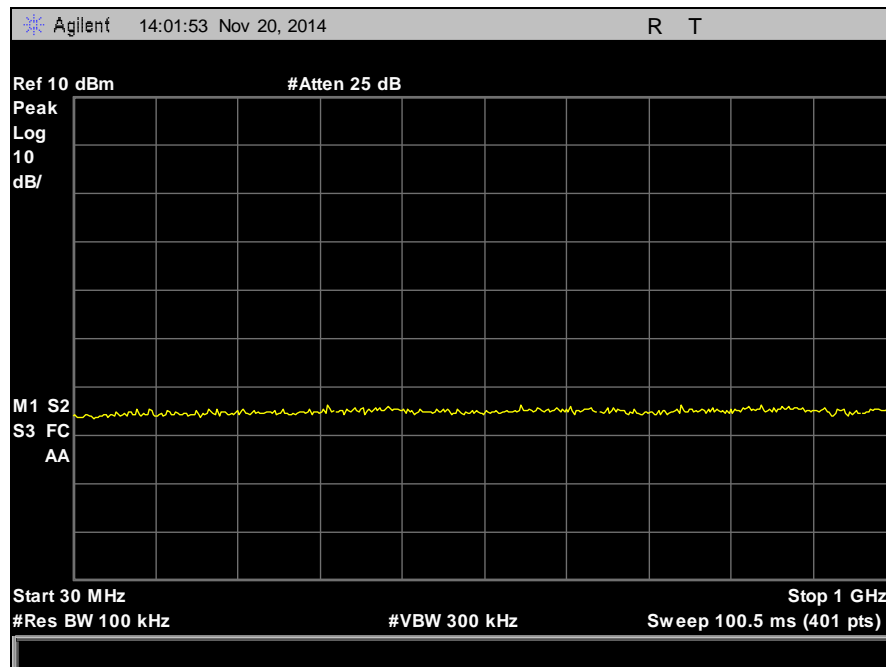
Plot 30. Conducted Spurious Emissions, Mid Channel, 30 MHz – 1 GHz
