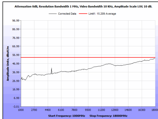
Plot 19. Radiated Spurious Emissions, Mid Channel, 1 GHz – 18 GHz, Average
