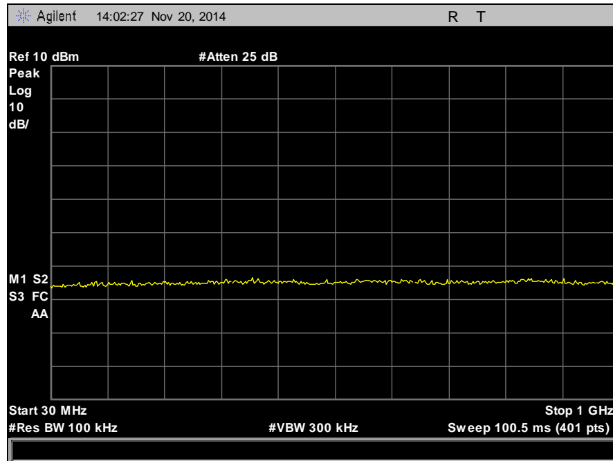
Plot 32. Conducted Spurious Emissions, High Channel, 30 MHz – 1 GHz
