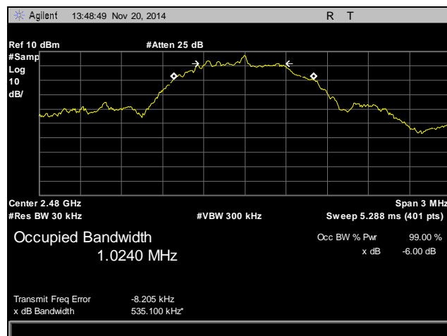
Plot 11. 99% Occupied Bandwidth, High Channel
