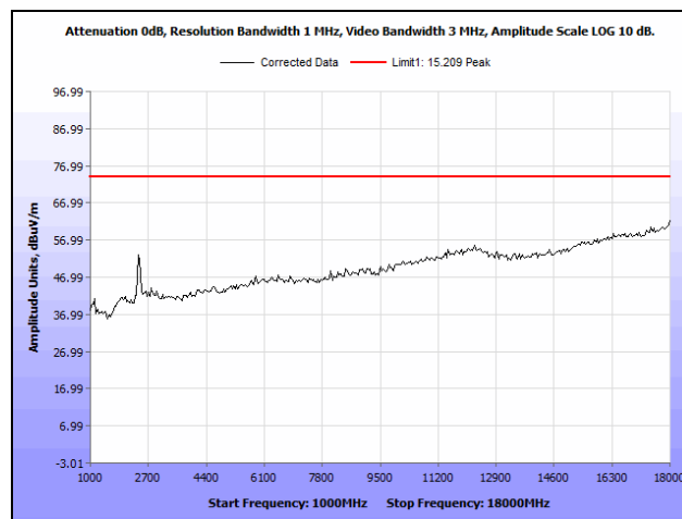
Plot 17. Radiated Spurious Emissions, Low Channel, 1 GHz – 18 GHz, Peak
