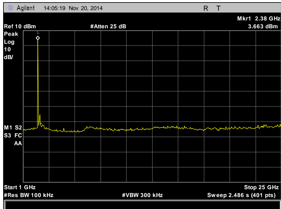
Plot 29. Conducted Spurious Emissions, Low Channel, 1 GHz – 25 GHz
