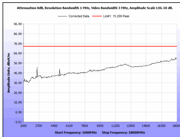
Plot 23. Radiated Spurious Emissions, High Channel, 1 GHz – 18 GHz, Peak
