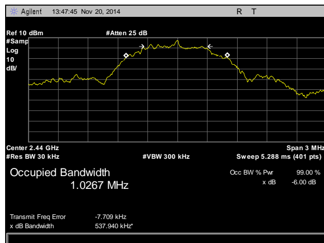
Plot 10. 99% Occupied Bandwidth, Mid Channel
