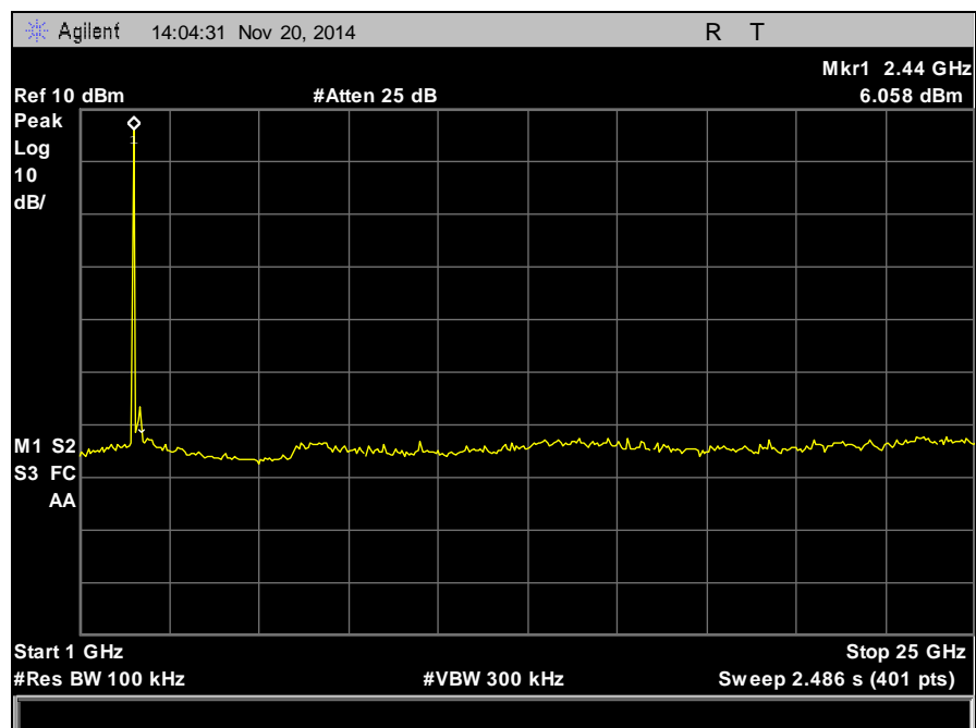
Plot 31. Conducted Spurious Emissions, Mid Channel, 1 GHz – 25 GHz
