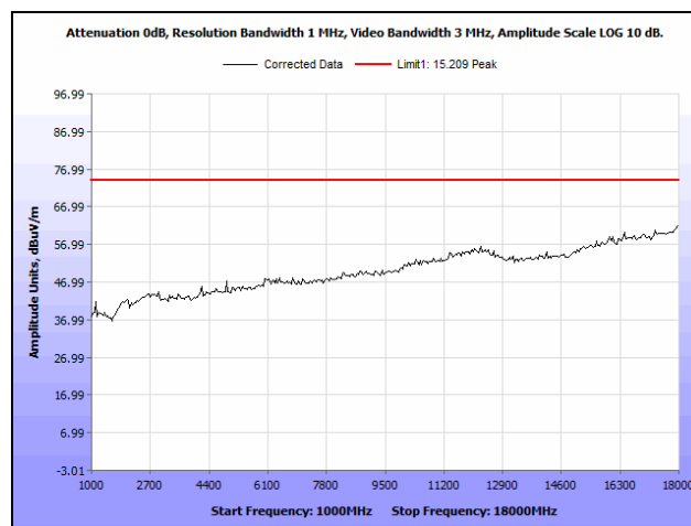
Plot 20. Radiated Spurious Emissions, Mid Channel, 1 GHz – 18 GHz, Peak
