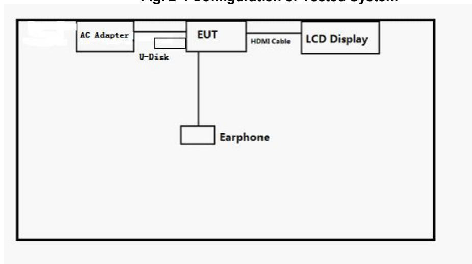
Fig. 2-1 Configuration of Tested System
