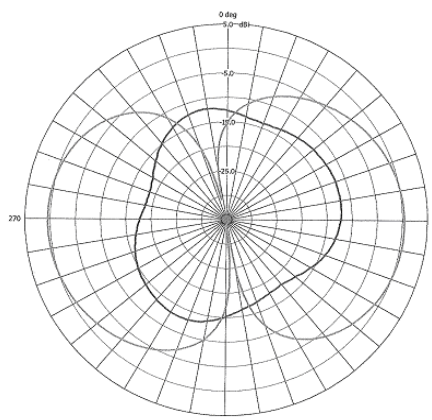
Elevation Plane Phi = 0 2.45 GHz
