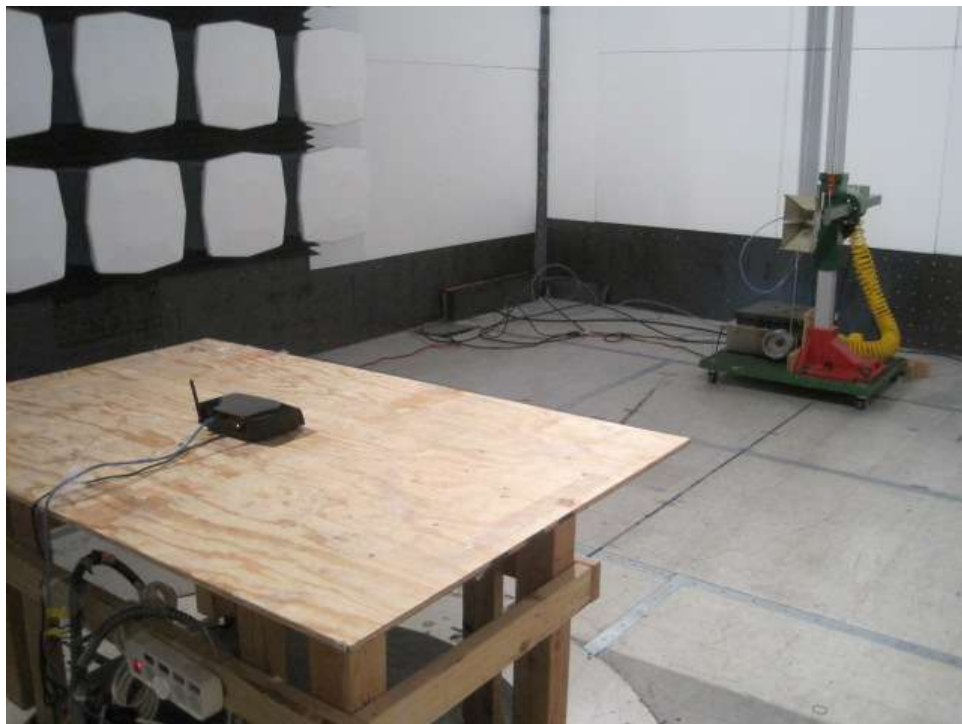
Radiated Emission (>1GHz) Setup Rear View
