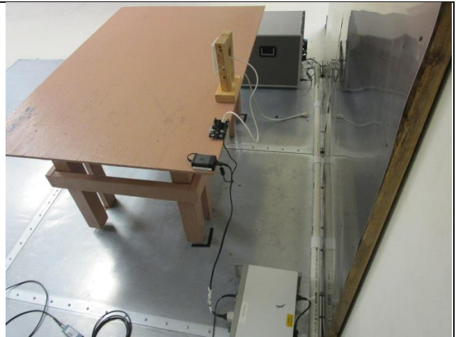
Conducted Emissions– Side View
