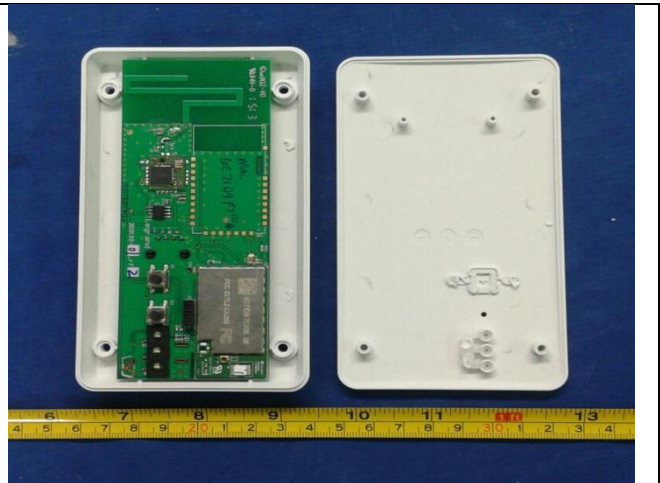
EUT-without cover
