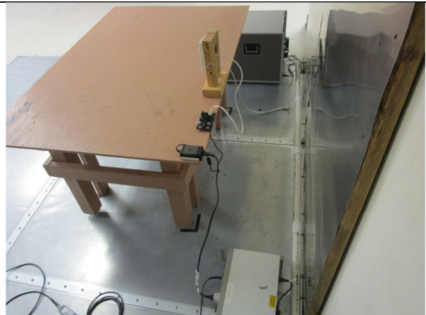
Conducted Emissions- Side View
