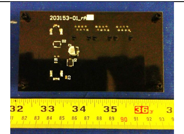
Power over CAT5 Module – Bottom View
