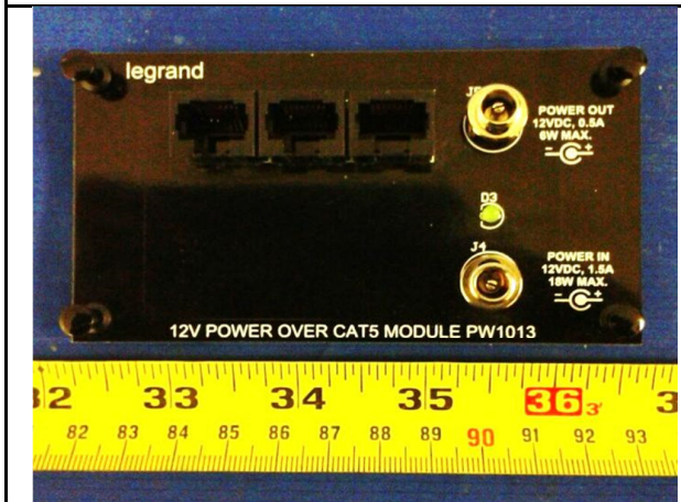
Power over CAT5 Module – Top View
