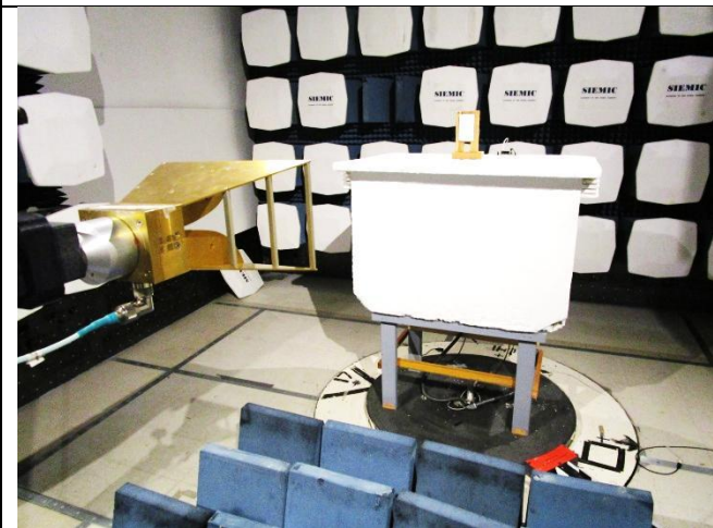
Spurious Emissions (>1GHz) – Front View
