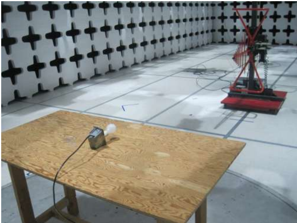
Radiated Emission Rear View (30MHz-1GHz)
