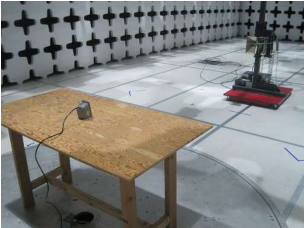
Radiated Emission (>1GHz) Setup Rear View
