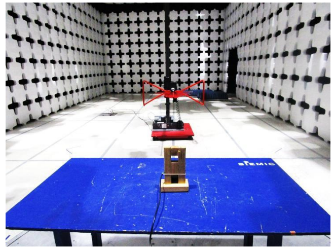
EUT Radiated Emissions (<1GHz) – Rear View
