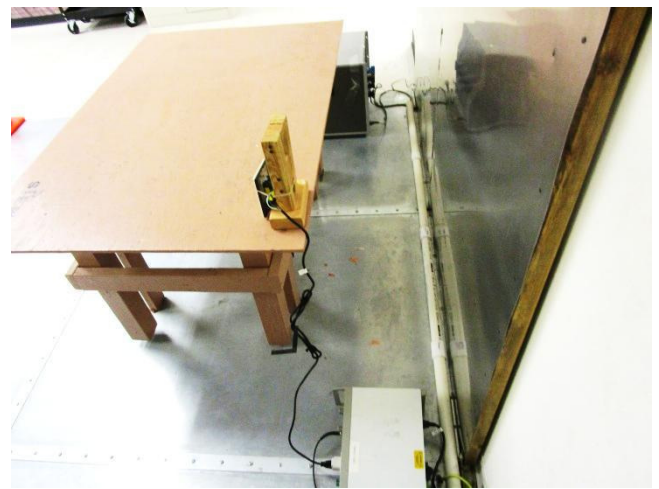
EUT AC Conducted Emission – Rear View
