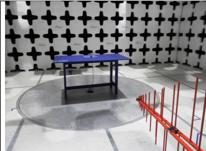
EUT with LC2103 Radiated Emissions (<1GHz) – Front View
