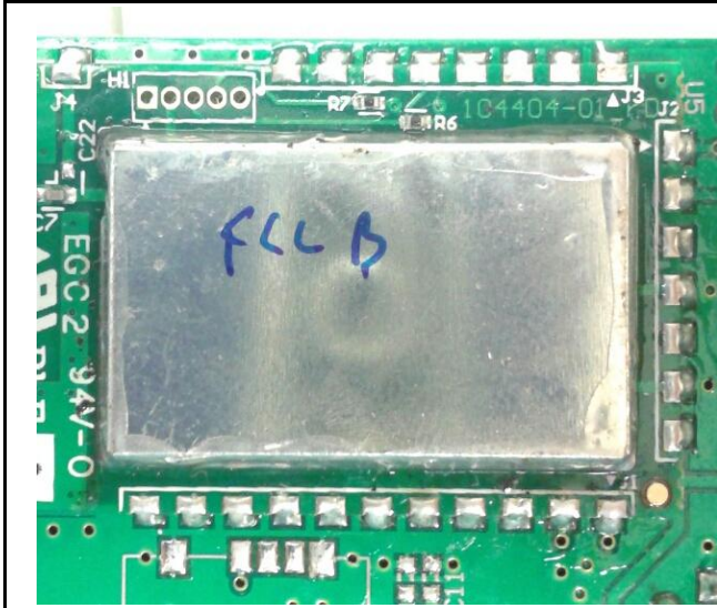
RFID Module With Shielding
