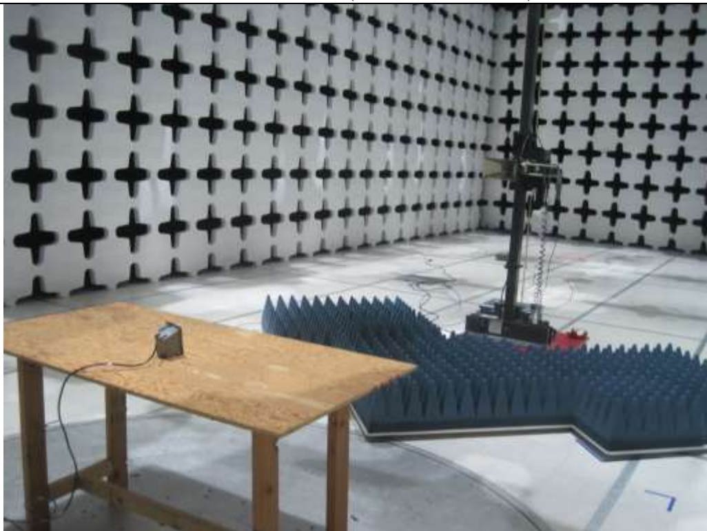
Radiated Emission above 1GHz (ADTP700RMUW1) - Rear View
