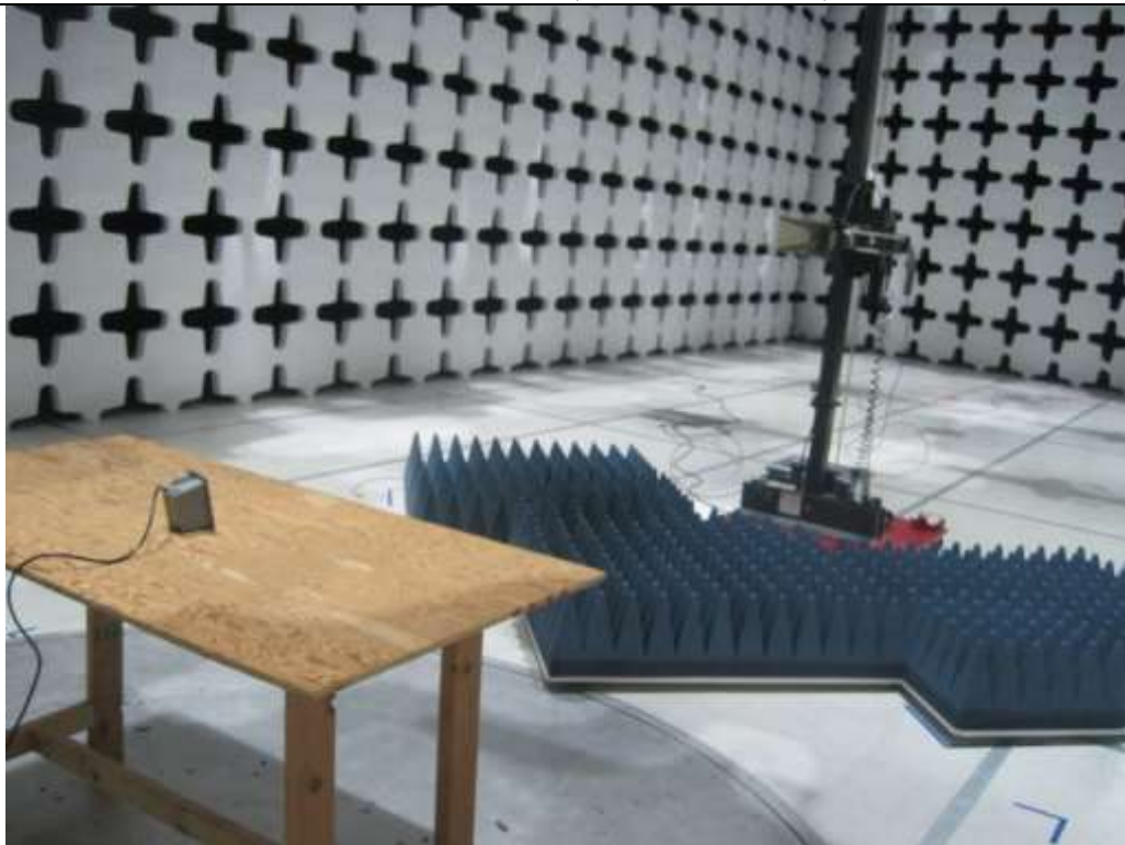
Radiated Emission above 1GHz (ASTP155RMW1) - Rear View
