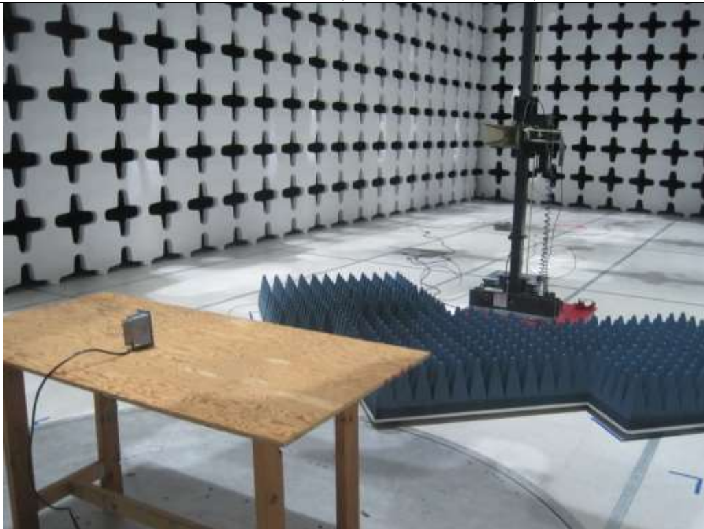
Radiated Emission above 1GHz (ADTH700RMTUW1) - Rear View
