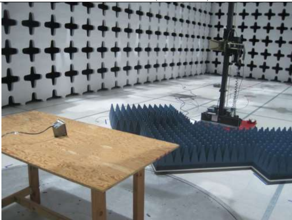
Radiated Emission above 1GHz (ASTHRRW1) - Rear View
