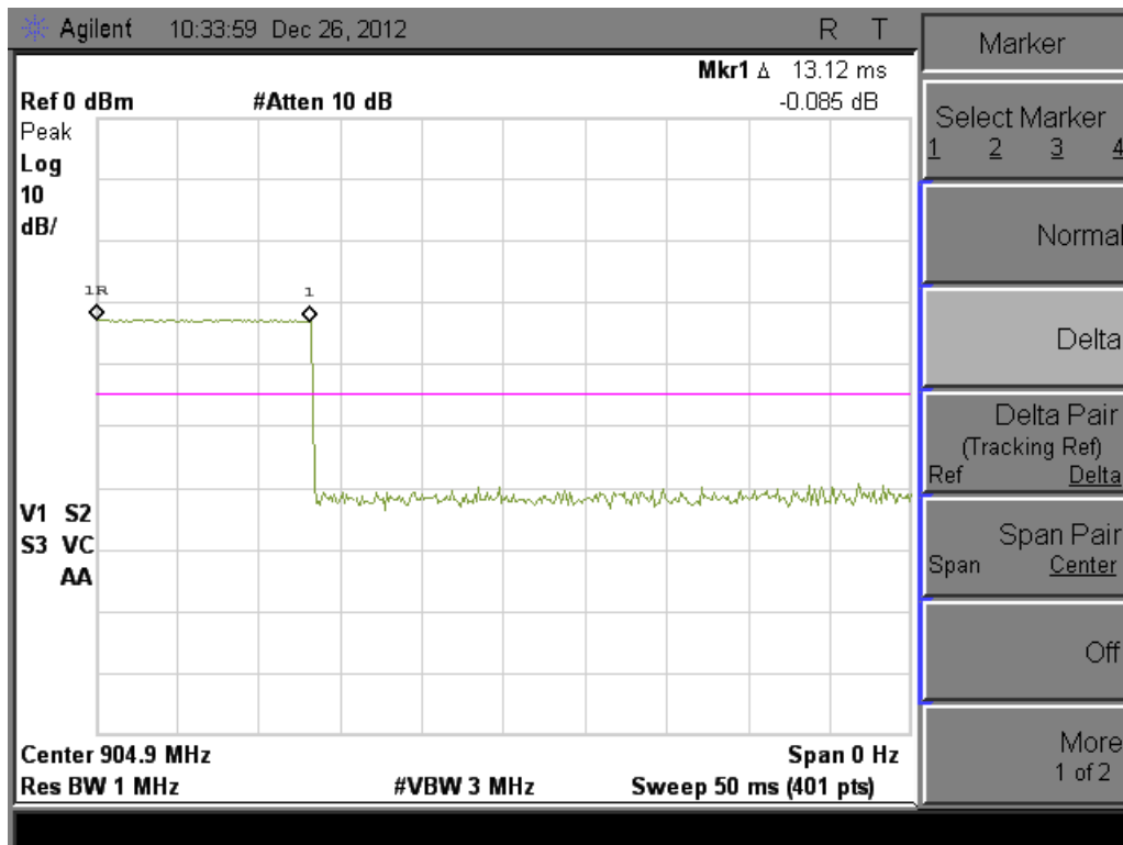
Plot - TX-Cycle time _Low CH
