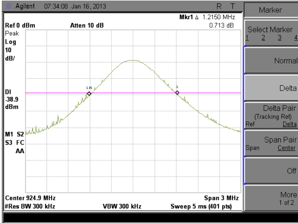
Plot - TX-924.873MHz-20dB BW
