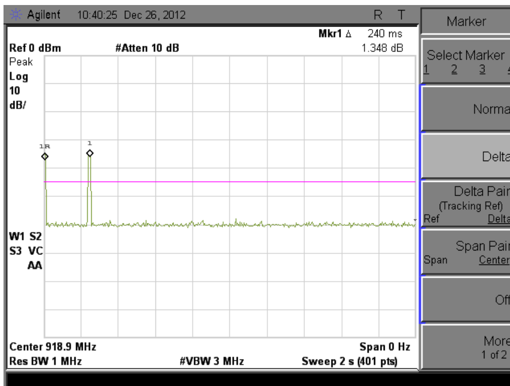
Plot - TX-Cycle time _Mid CH
