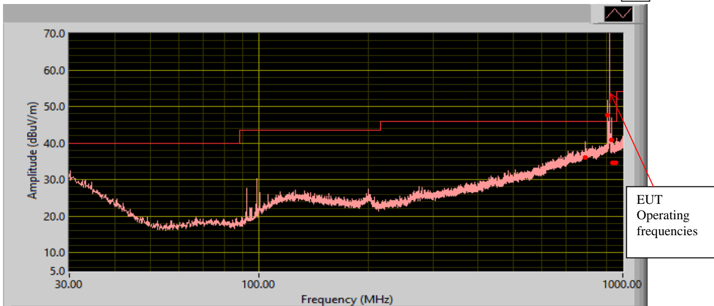
Below 1GHz Emission Test Data @ 3M
