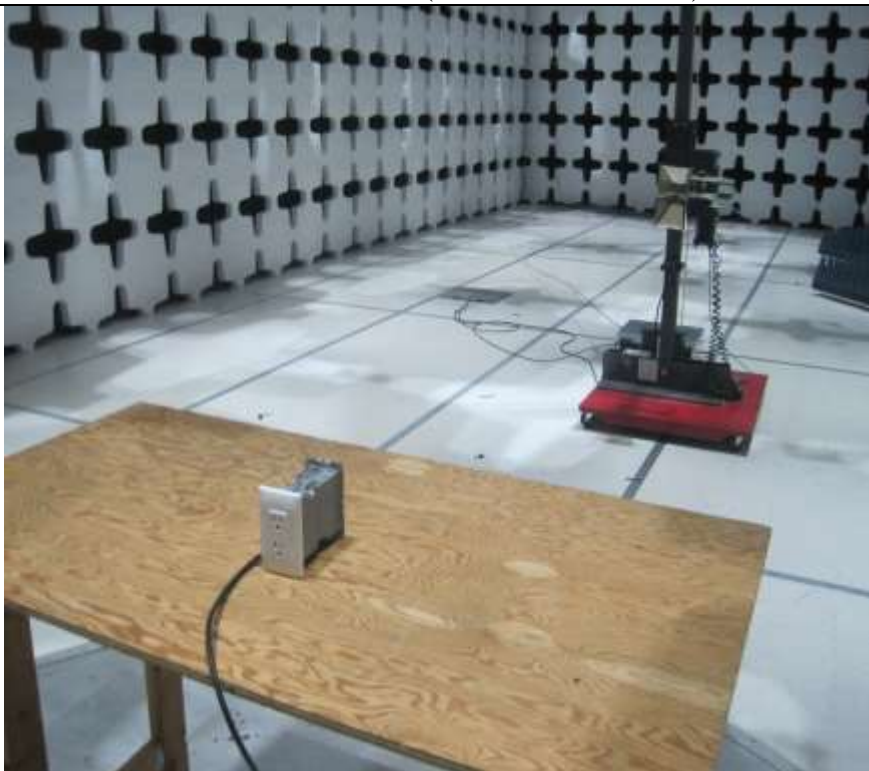
Radiated Emission above 1GHz (ADTP700MMHW2) - Rear View
