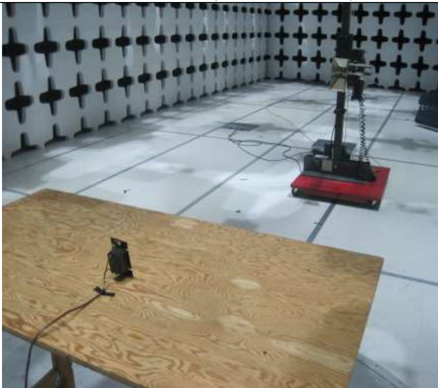
Radiated Emission above 1GHz (ADTH700MMUW2) - Rear View
