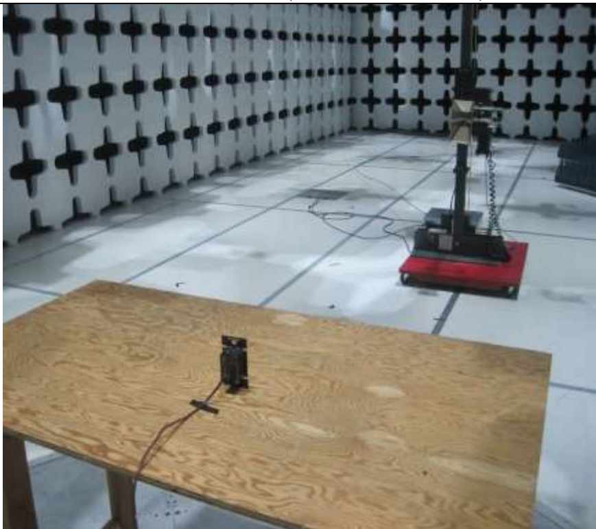
Radiated Emission above 1GHz (ADWR700MMUW2) - Rear View
