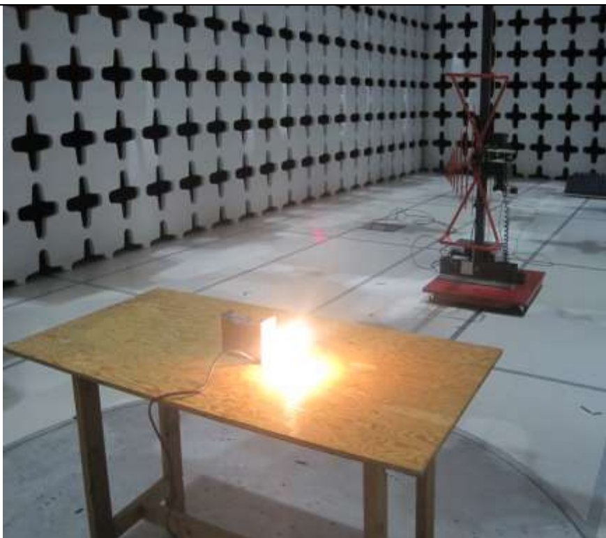
Radiatd Emission below 1GHz - Rear View
