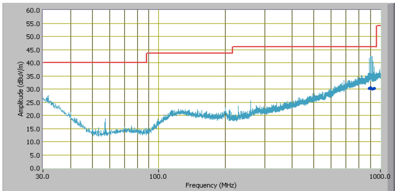
Below 1GHz Emission Test Data @ 3M
