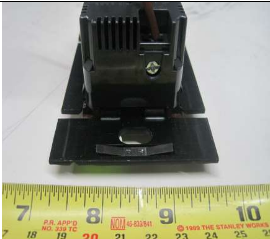
ADTH700MMUW2-Rear
