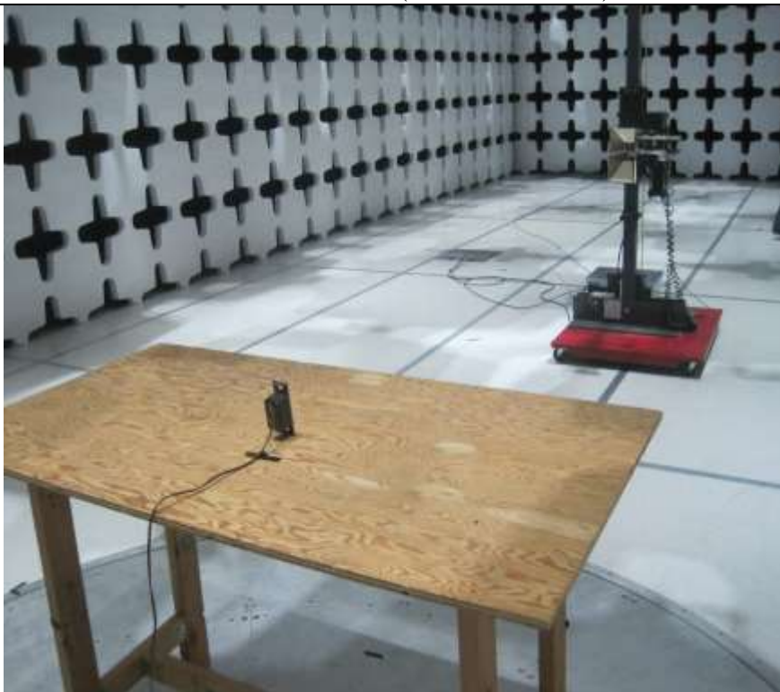
Radiated Emission above 1GHz (ADWRMRUW2) - Rear View
