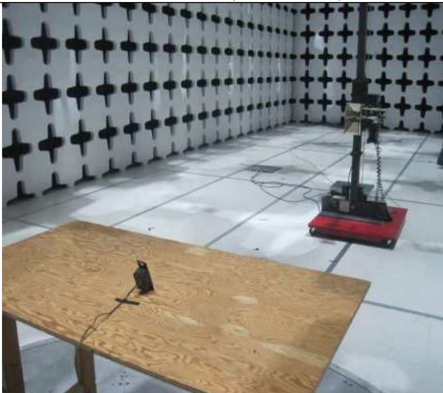
Radiated Emission above 1GHz (ADTPMRUW2) - Rear View
