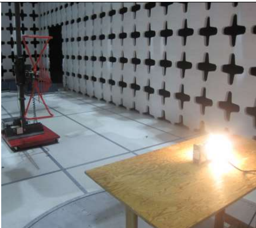
Radiated Emission below 1GHz - Rear View
