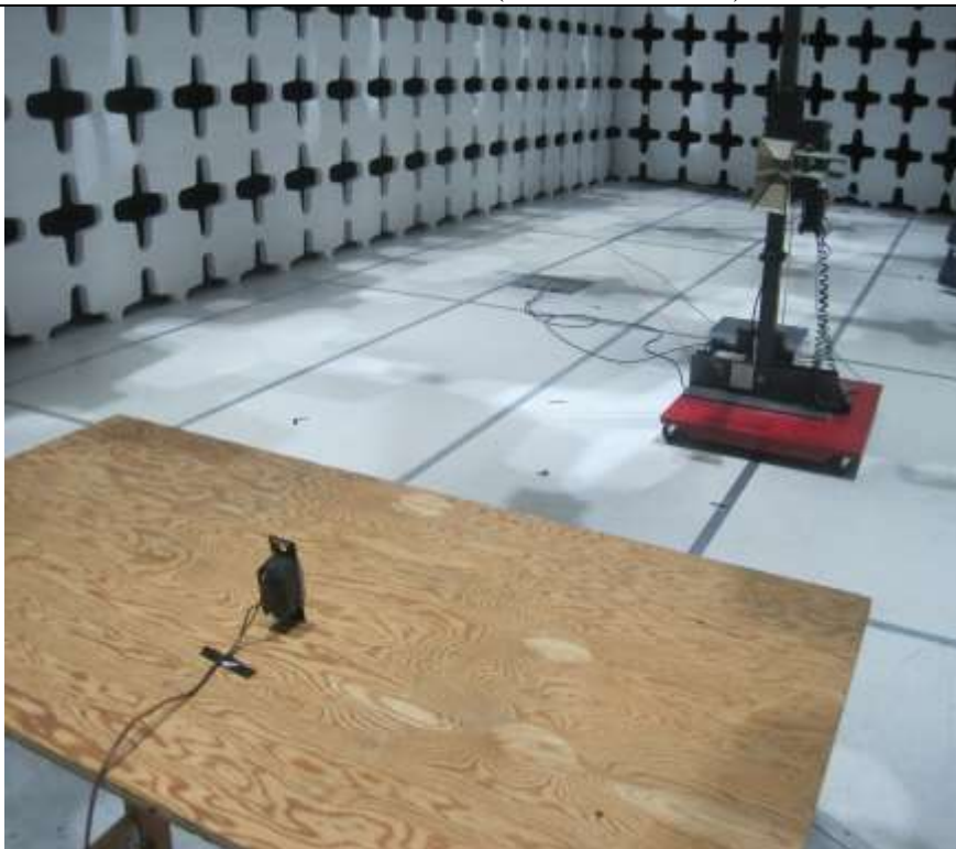
Radiated Emission above 1GHz (ADTHMRUW2) - Rear View
