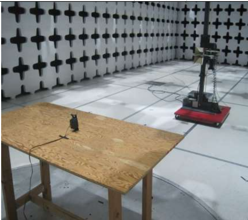
Radiated Emission above 1GHz (ASTPRF2W2) - Rear View
