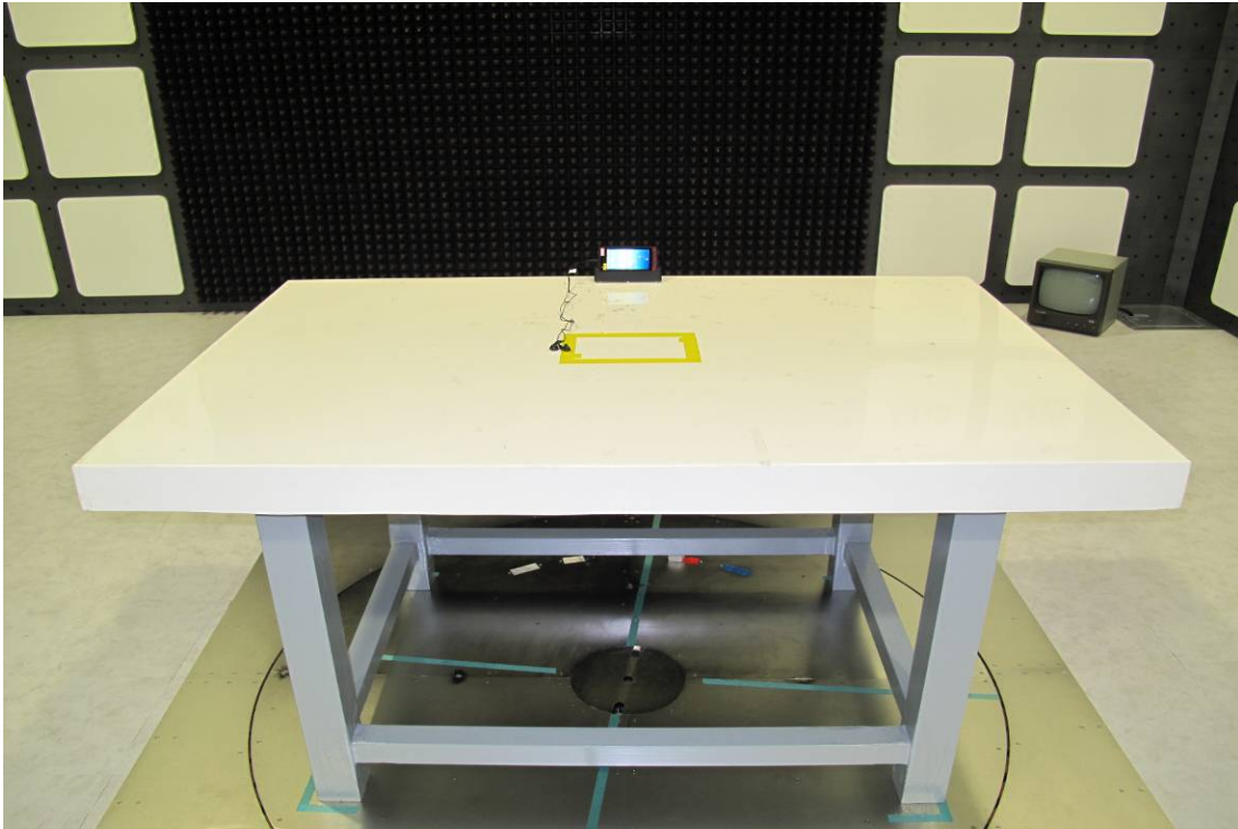
Radiated Emission Test Setup Photo (config 1)
