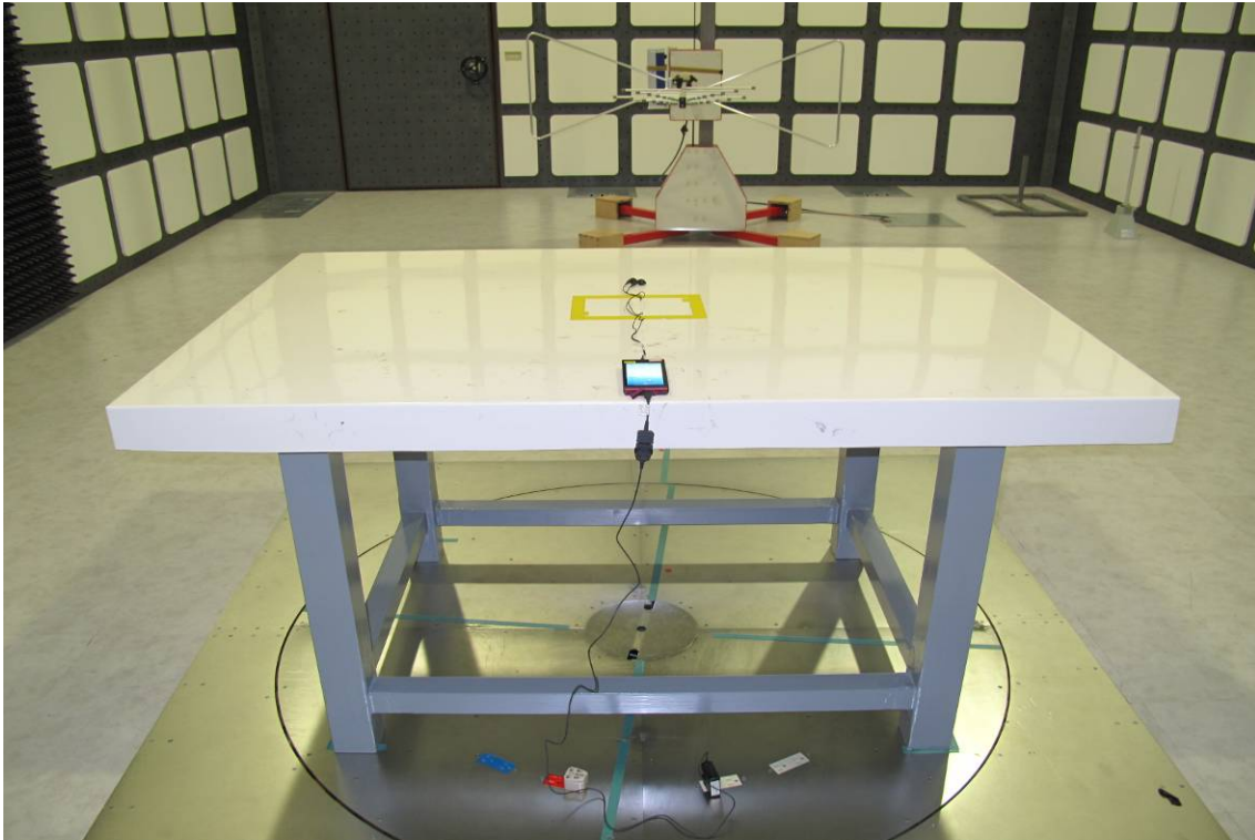
Radiated Emission Test Setup Photo (config 2, 3)
