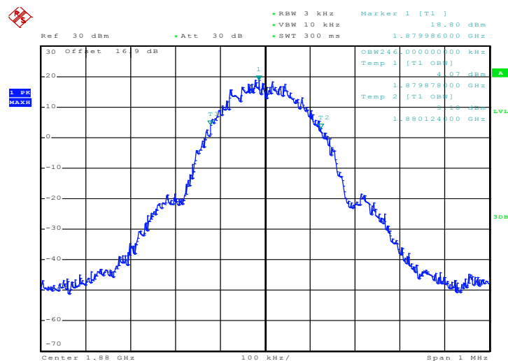
99% Occupied Bandwidth Plot on Channel 661
