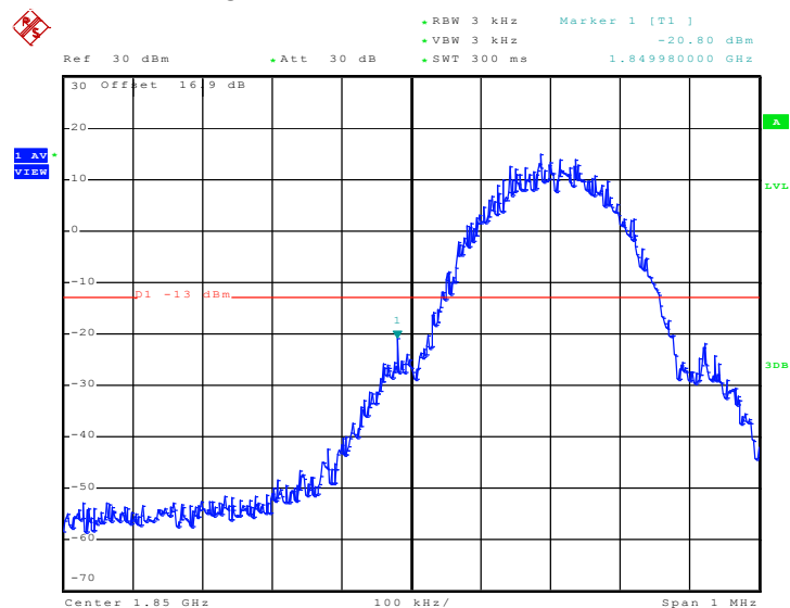
Lower Band Edge Plot on Channel 512
