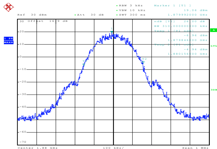
26dB Bandwidth Plot on Channel 661
