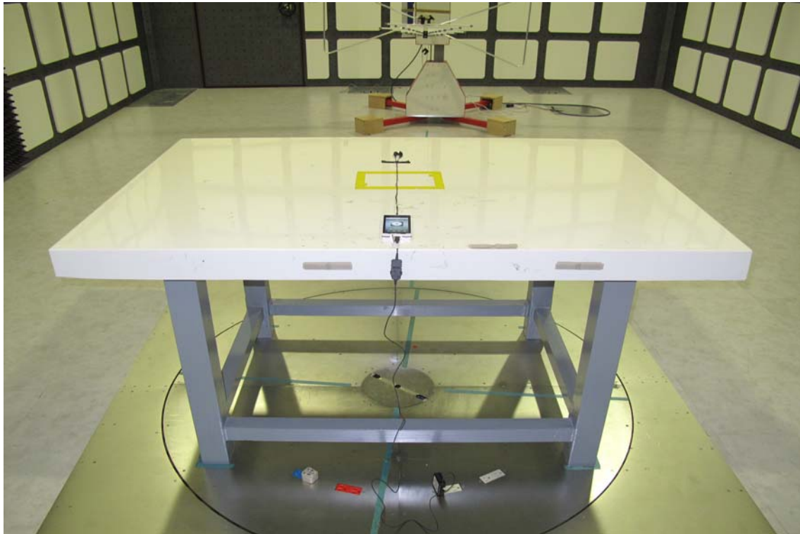
Radiated Emission Test Setup Photo (config 1, 2)
