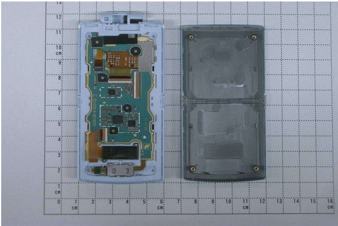
Upper Inner case (back) and Upper Outer case
