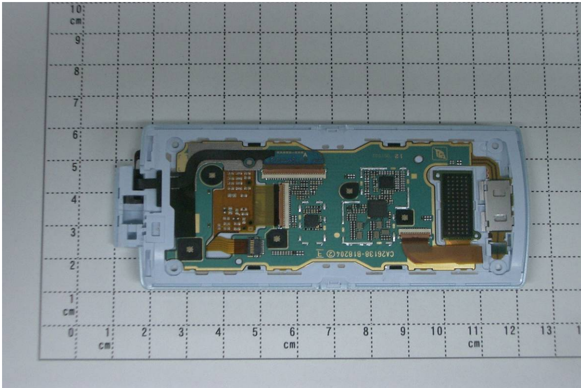
Upper Inner case (back) with Upper PCB
