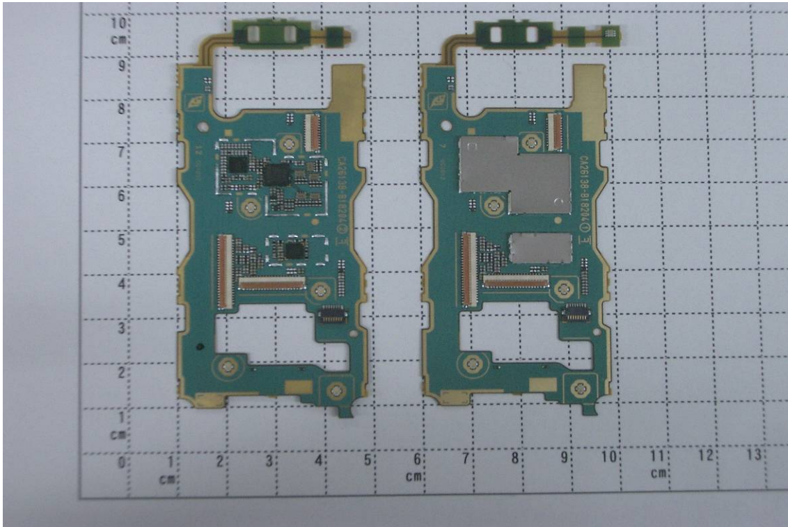
SUB Display (Front)
