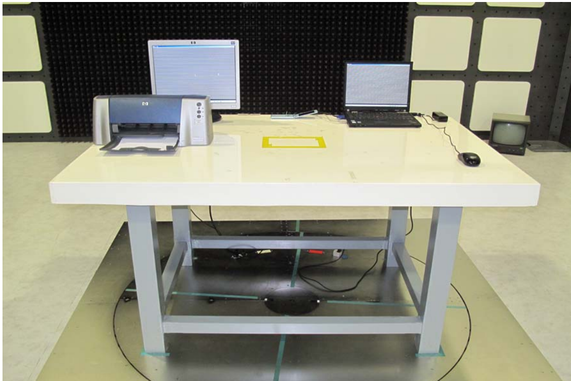
Radiated Emission Test Setup Photo (config 5)
