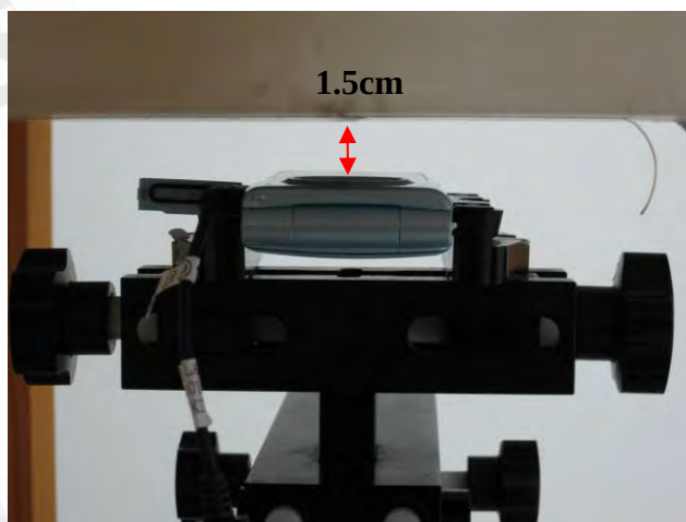
Fig.9 Body worn- EUT front to flat phantom and distance between flat phantom and mobile phone is 1.5 cm_ repeated with Headset.
