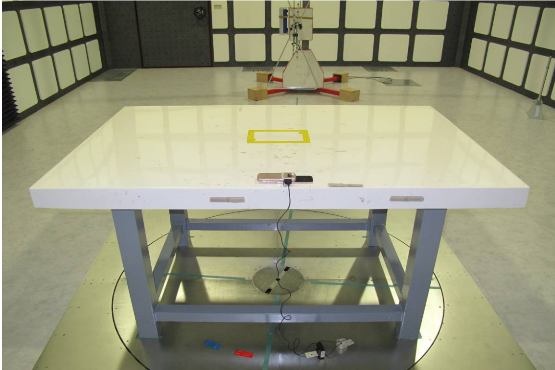
Radiated Emission Test Setup Photo (config 1, 3)
