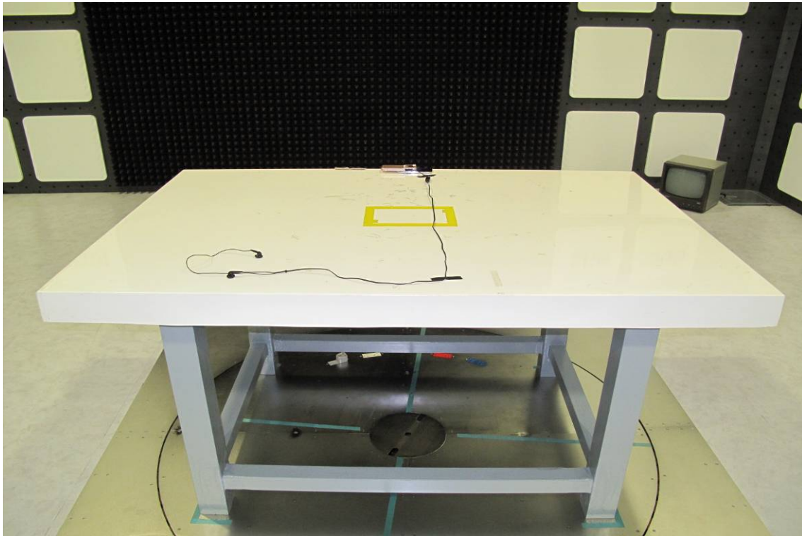
Radiated Emission Test Setup Photo (config 2, 4)
