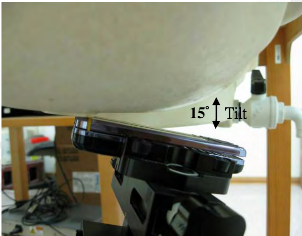
Fig.4 Right Head Section / Ear-Tilt Position(15°)_ Slider off
