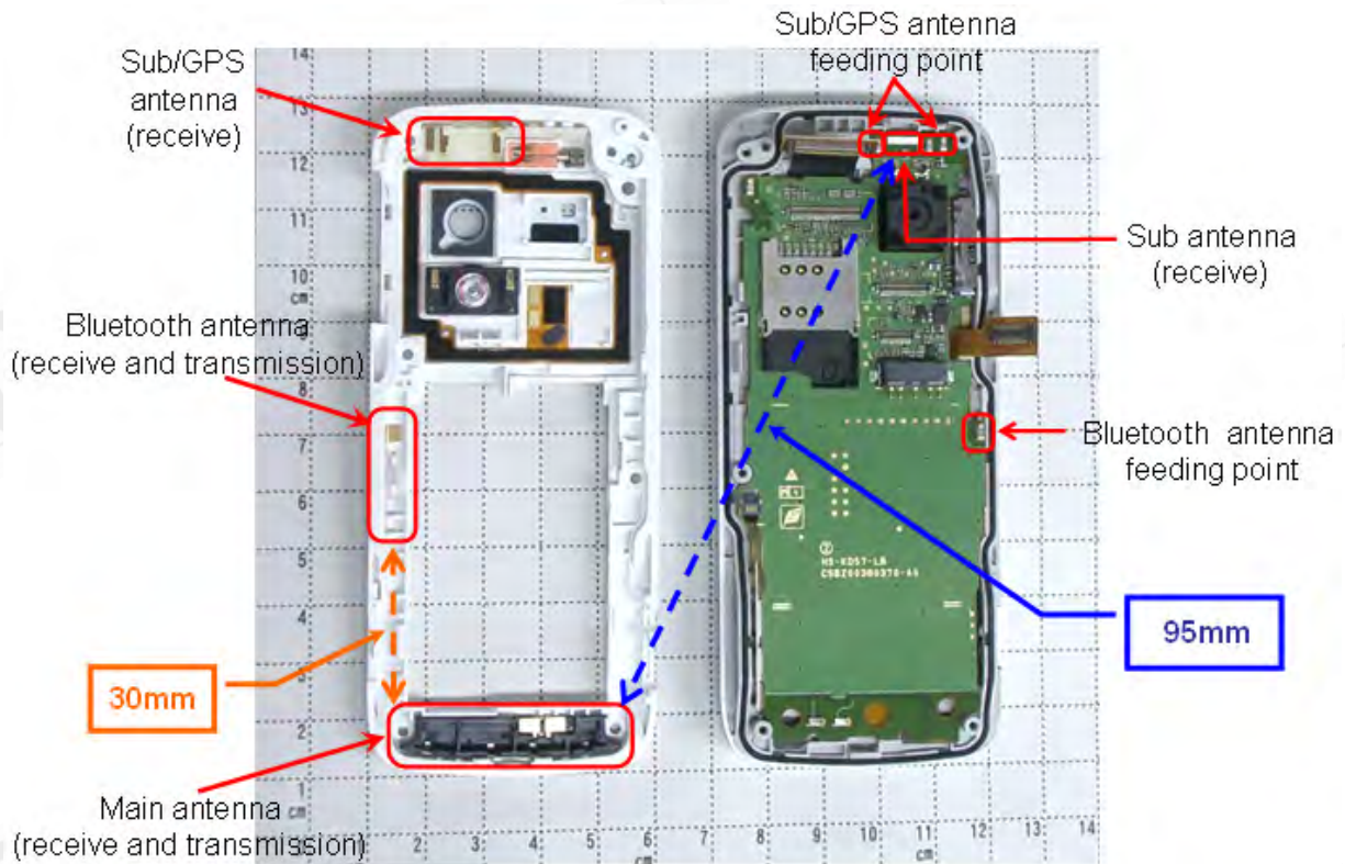
Fig.16 Antenna position of EUT
