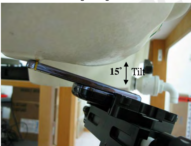
Fig.8 Right Head Section / Ear-Tilt Position(15°)_ Slider on
