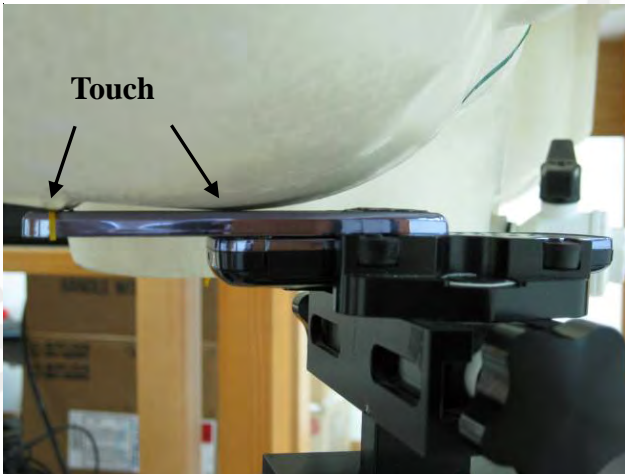
Fig.7 Right Head Section / Cheek-Touch Position_ Slider on
