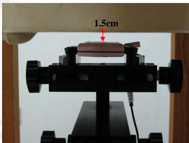
Fig.9 Body worn- EUT back to flat phantom and distance between flat phantom and mobile phone is 1.5 cm_ repeated with headset.
