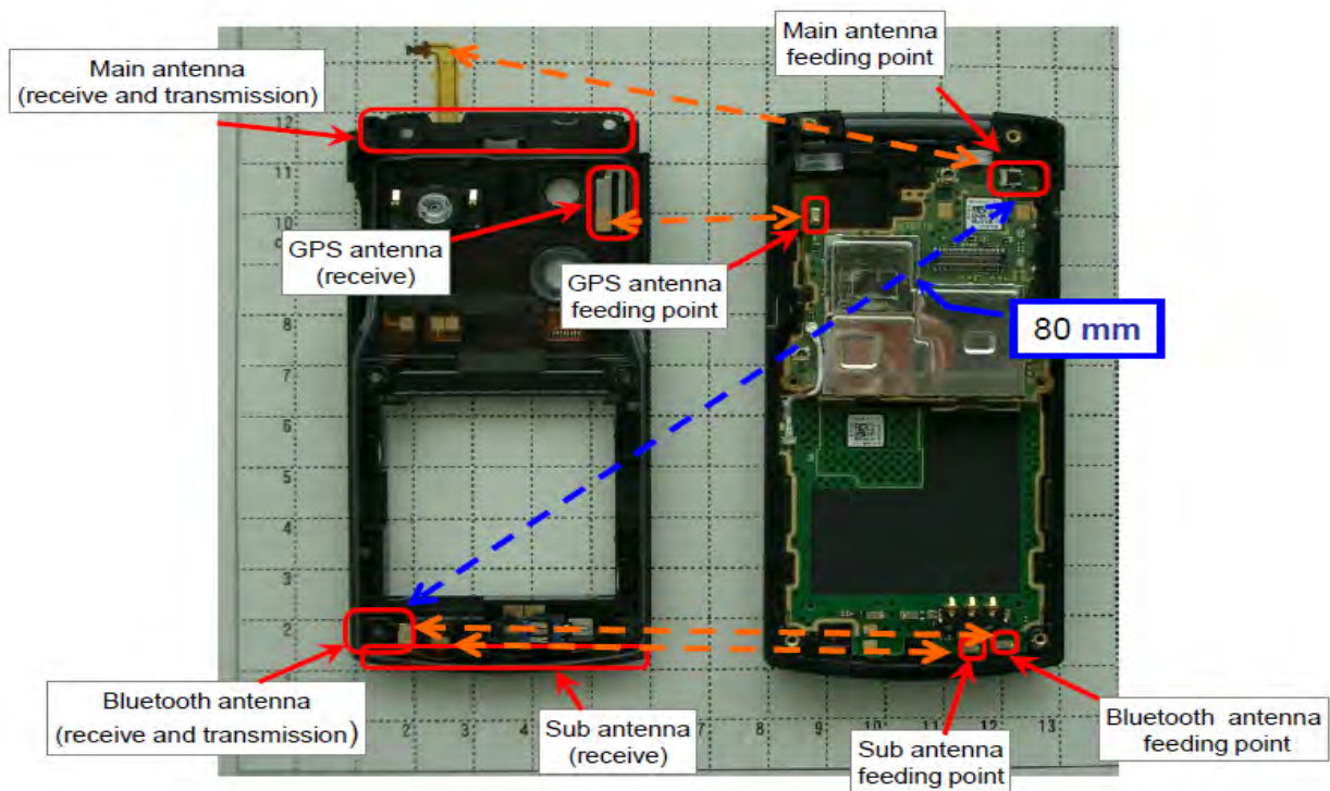
Fig.16 Antenna position of EUT
