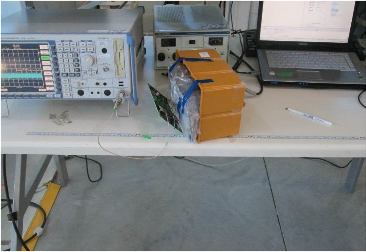
Test setup photo 5 Conducted measurements
