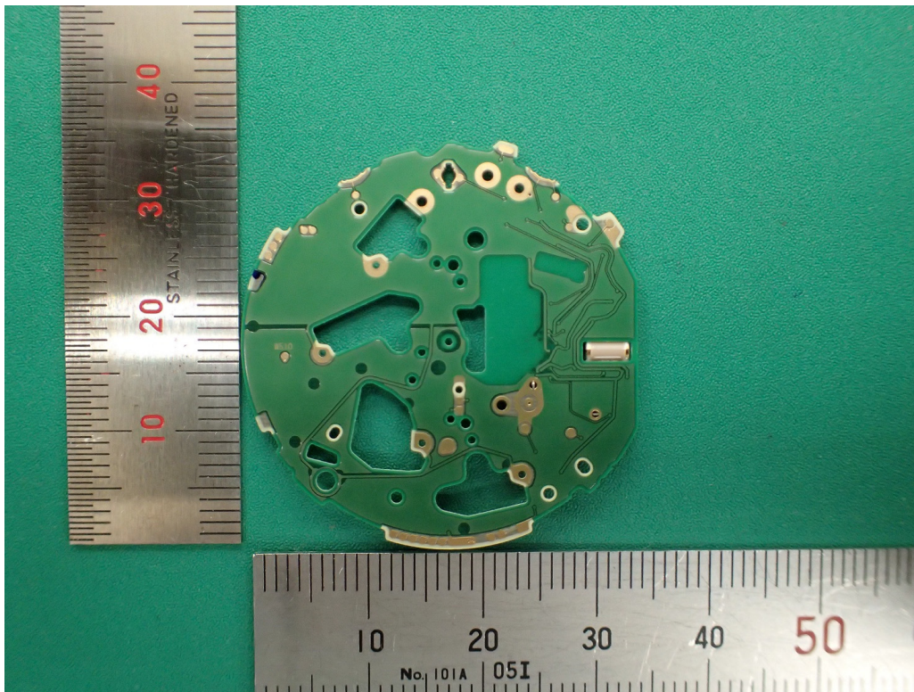
PCB Bottom (with shield)
