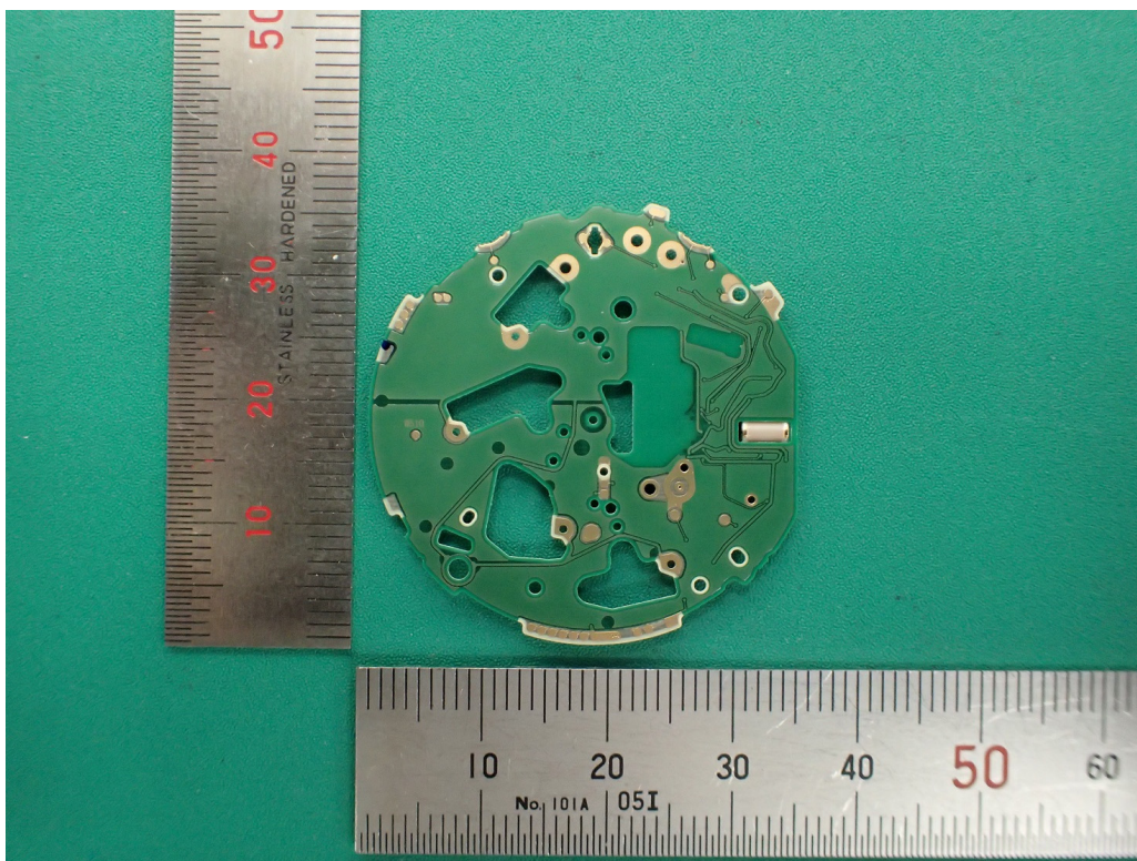
PCB Bottom (without shield)
