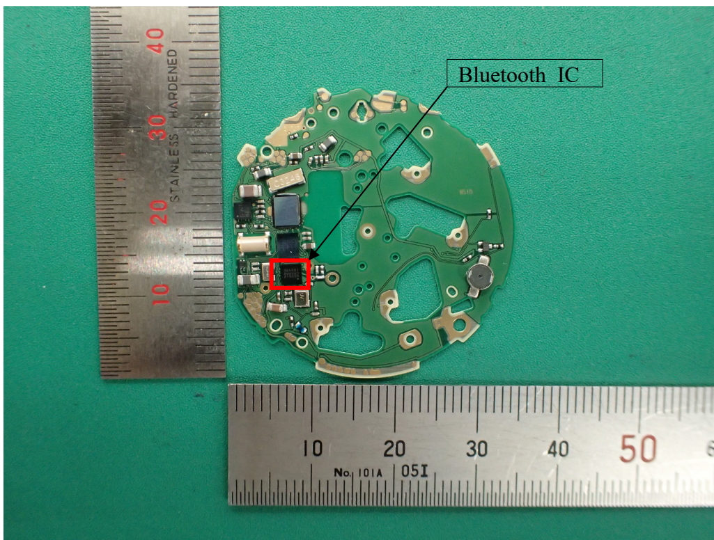
PCB Top (without shield)
