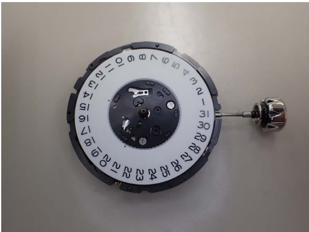
Module without Solar cell and Antenna
