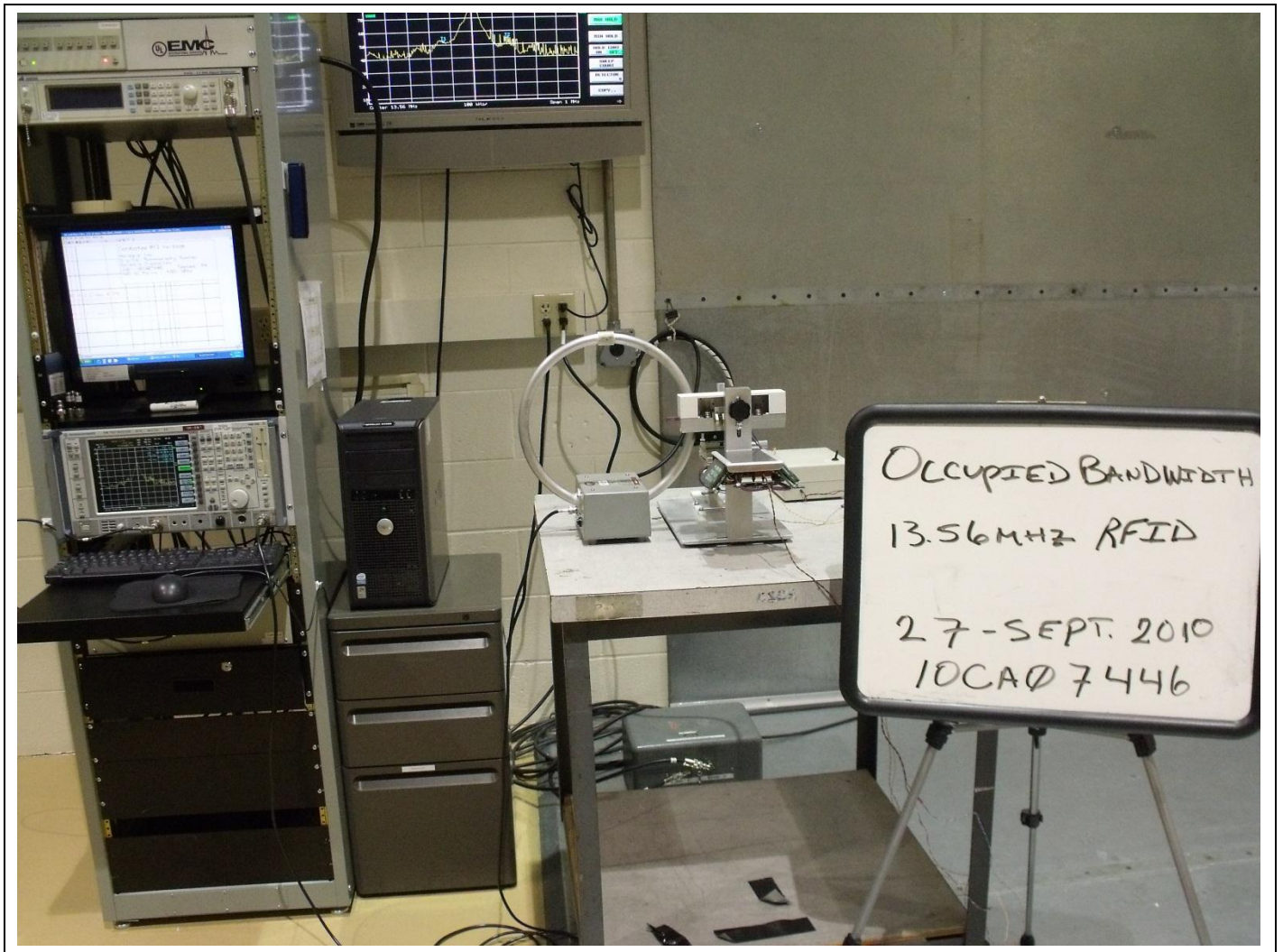
Test Setup for Occupied Bandwidth
