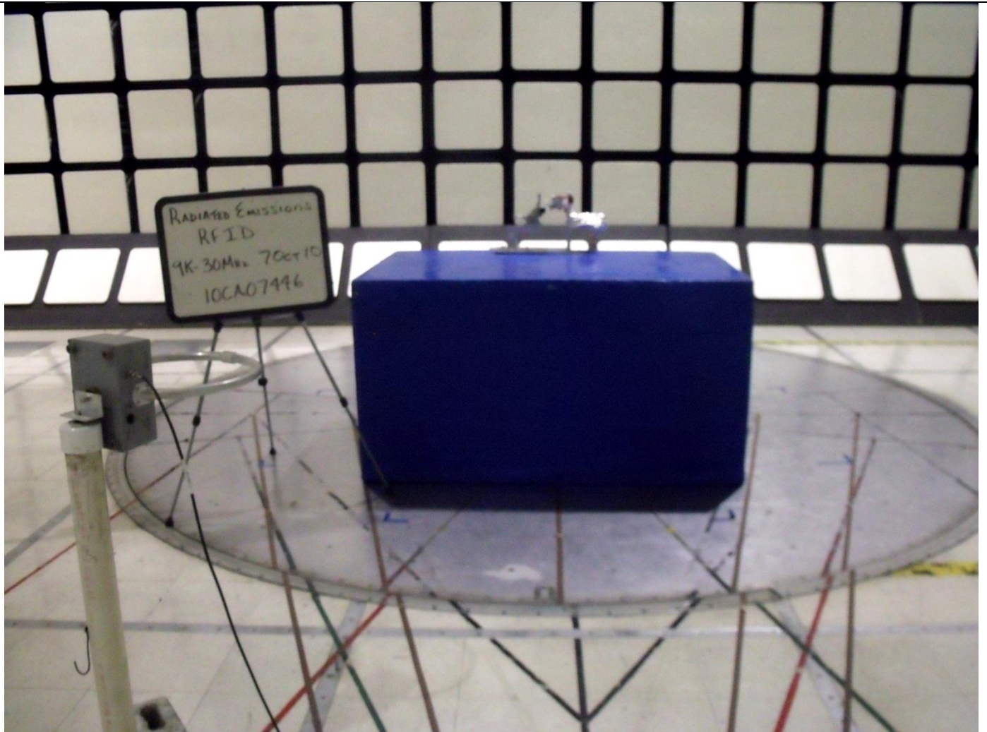
9KHz to 30 MHz Horizontal Polarity Front View
