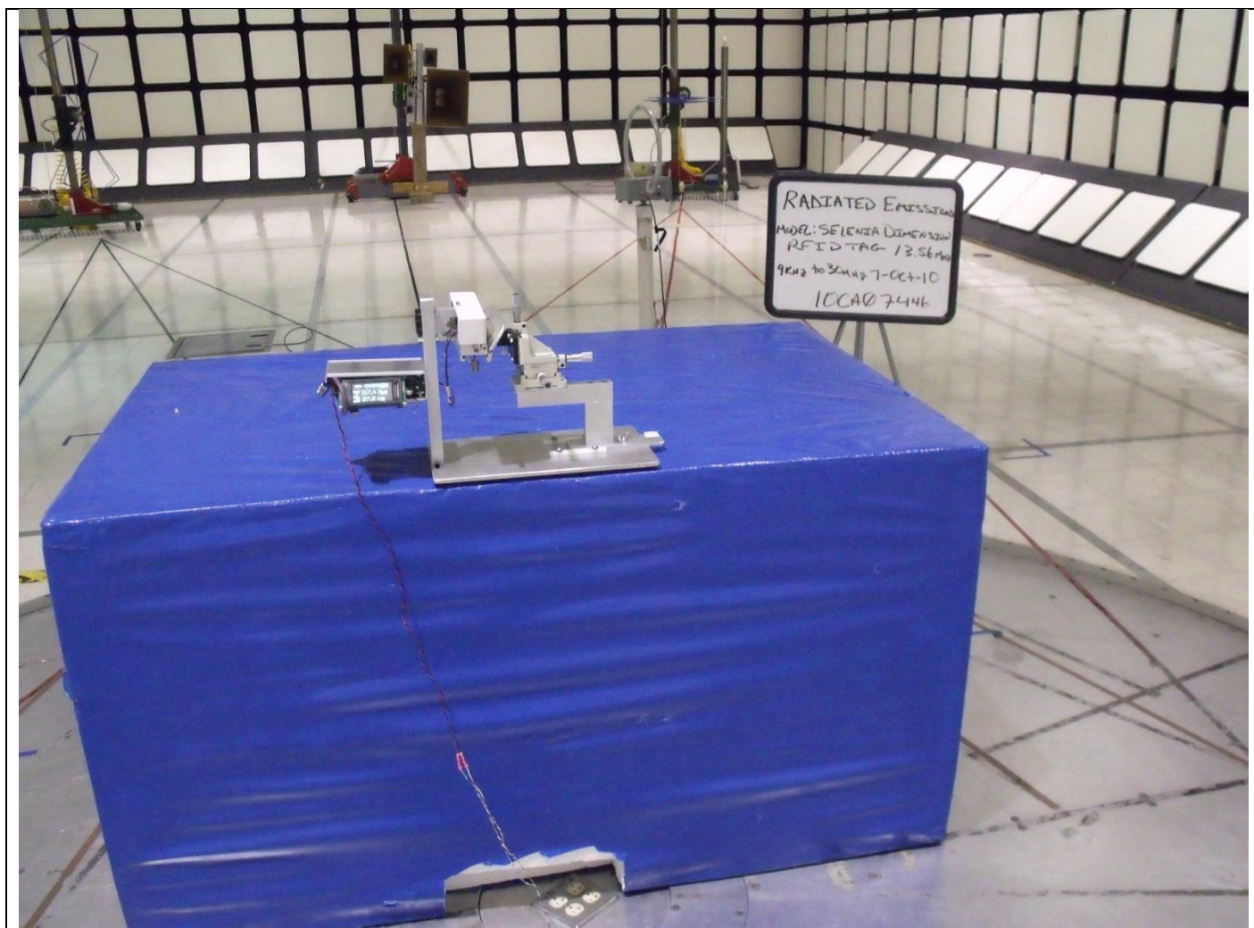
9KHz to 30 MHz Vertical Polarity Rear View
