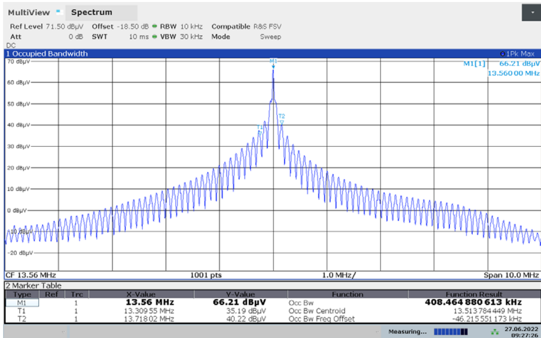
Plot 1: 99 % emission bandwidth
