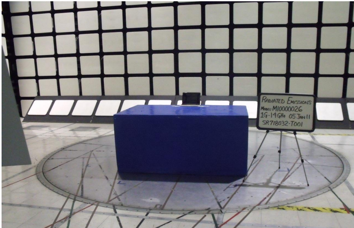
1 to 14GHz, Front View
