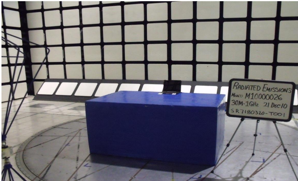
30 to 1000MHz Front View
