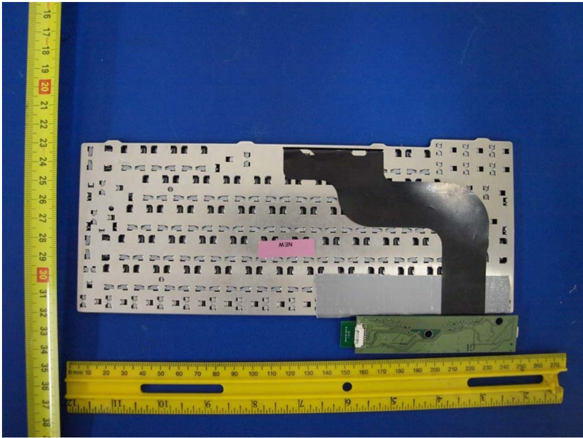
Bottom View of Keyboard
