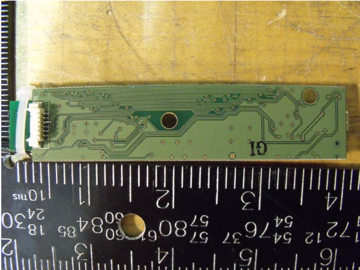
Bottom View of PCBA
