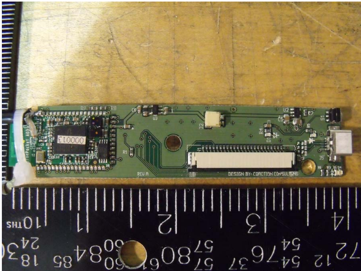
Top View of PCBA
