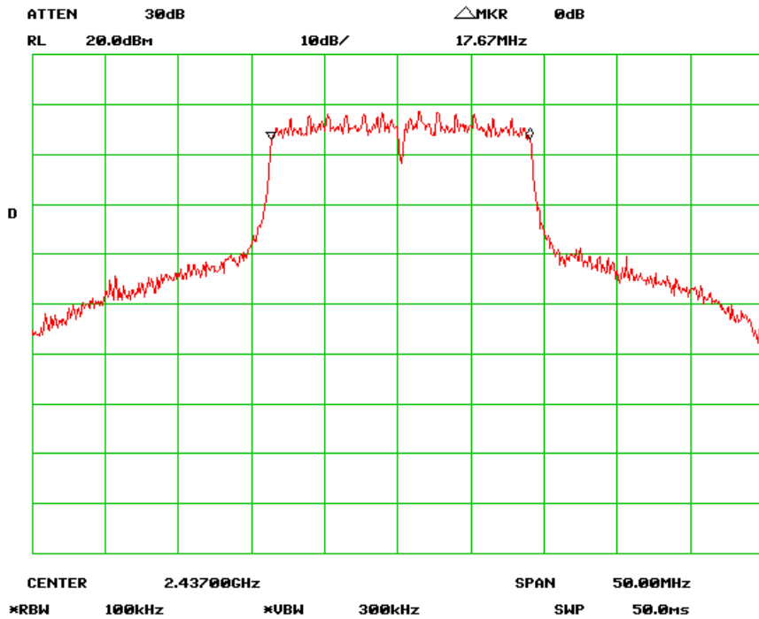
6dB Bandwidth – Mid Channel (802.11n-20MHz)
