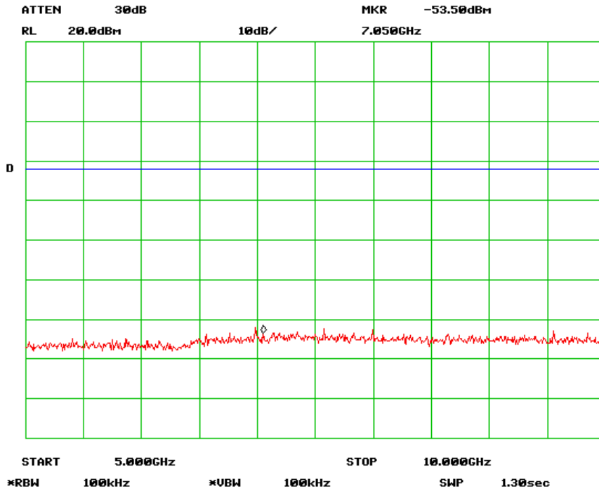
Antenna Port Emission Mid-3 Channel (802.11g)
