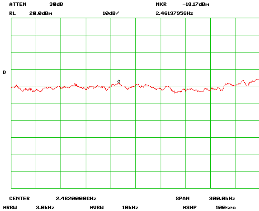
PSD - High Channel (802.11n-20MHz)
