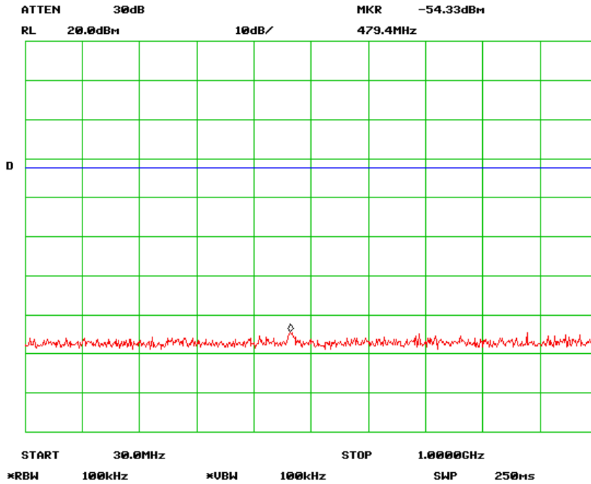
Antenna Port Emission Low-1 Channel (802.11n 20MHz)
