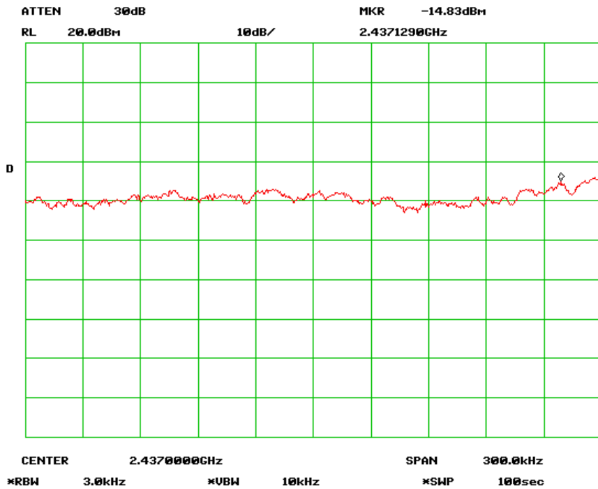
PSD - Mid Channel (802.11n-20MHz)
