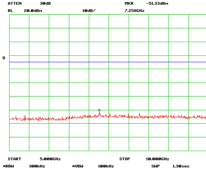
Antenna Port Emission Low-3 Channel (802.11n 40MHz)
