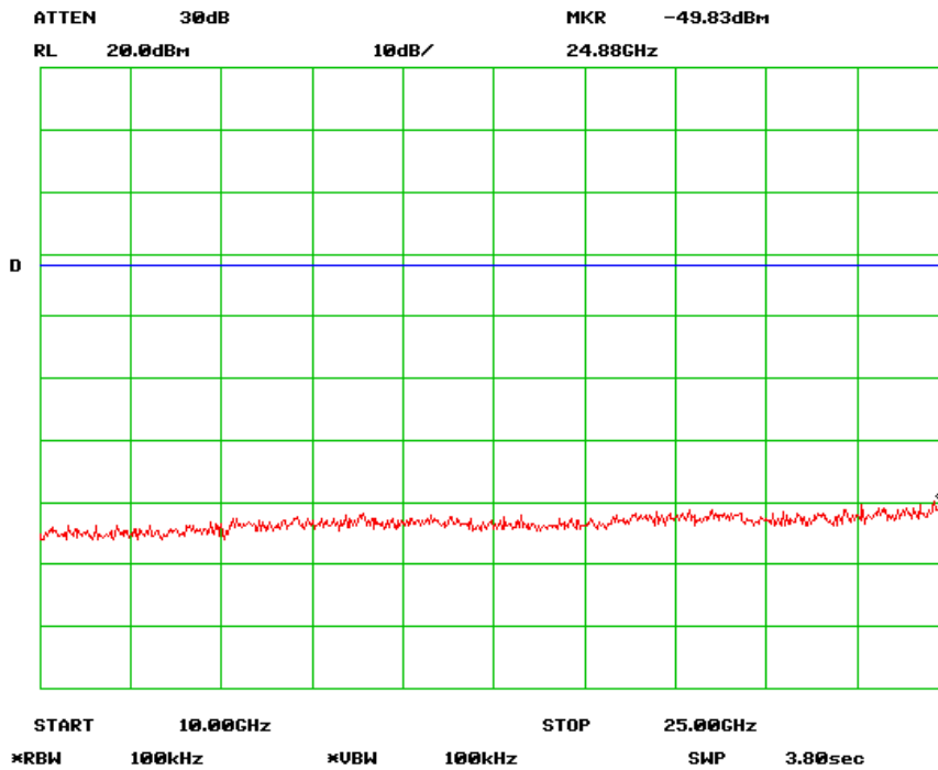
Antenna Port Emission Low-4 Channel (802.11g)
