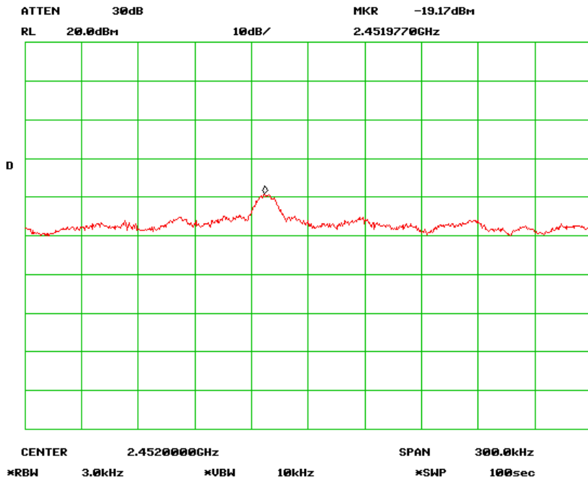
PSD - High Channel (802.11n-40MHz)
