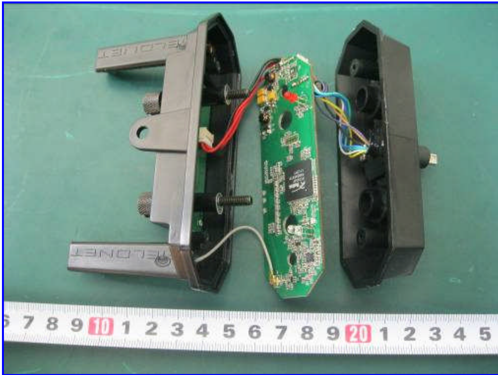
Front View of EUT Cover off
