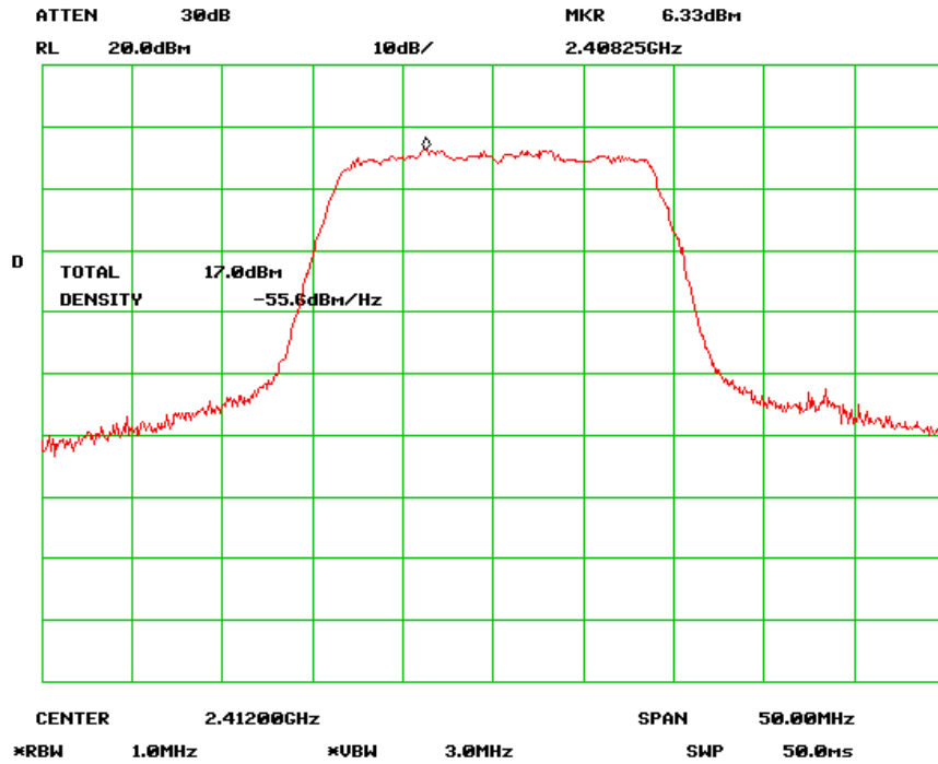
Output Power Low Channel (802.11n-20MHz)
