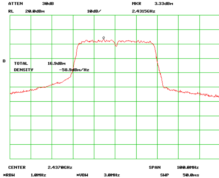
Output Power Mid Channel (802.11n-40MHz)
