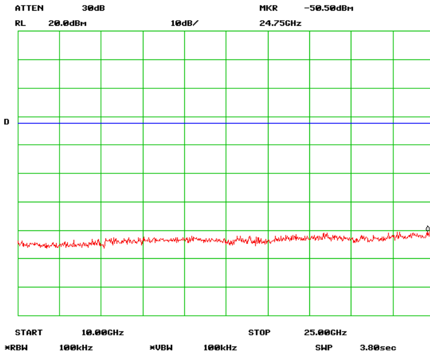
Antenna Port Emission Mid-4 Channel (802.11n 20MHz)
