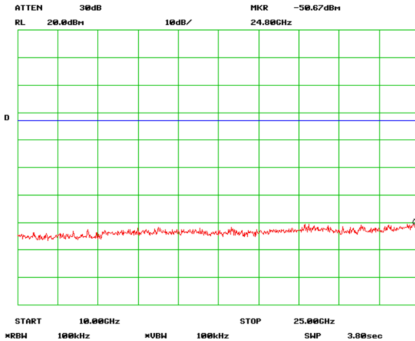
Antenna Port Emission High-4 Channel (802.11n 20MHz)
