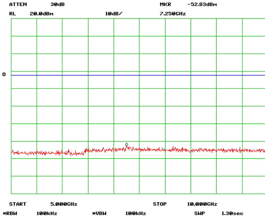
Antenna Port Emission Mid-3 Channel (802.11n 20MHz)
