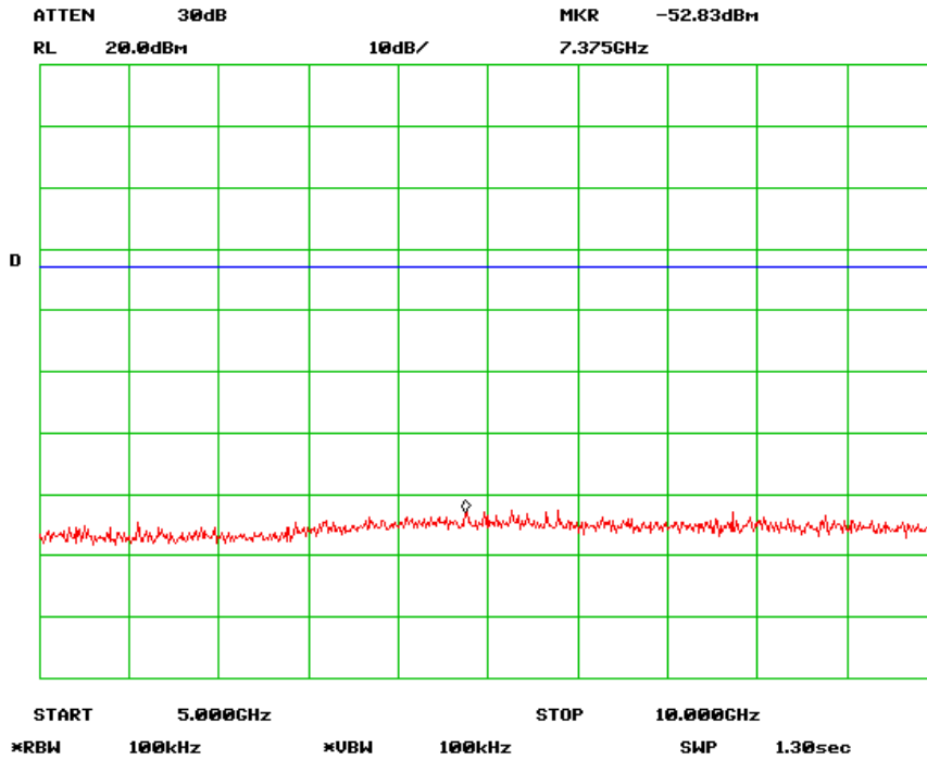
Antenna Port Emission High-3 Channel (802.11n 20MHz)
