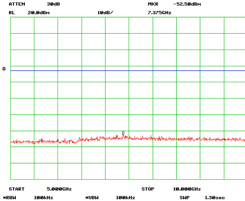
Antenna Port Emission High-3 Channel (802.11g)
