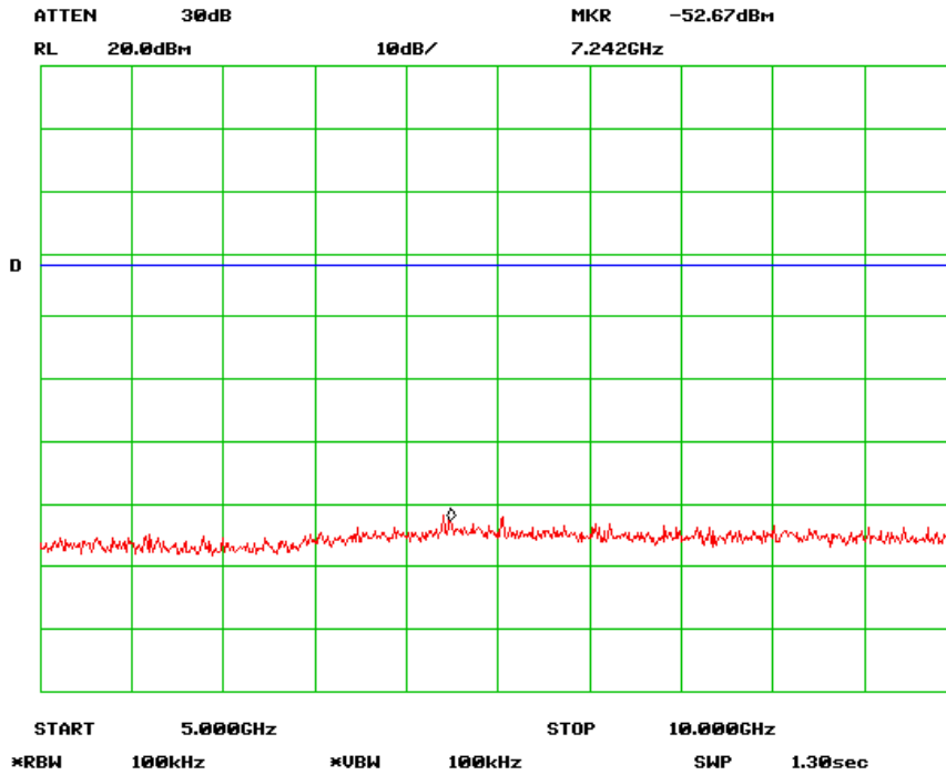
Antenna Port Emission Low-3 Channel (802.11n 20MHz)
