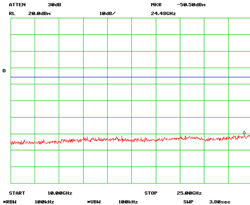
Antenna Port Emission High-4 Channel (802.11n 40MHz)
