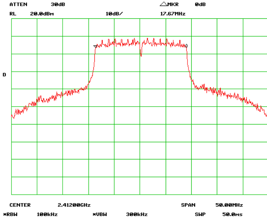
6dB Bandwidth – Low Channel (802.11n-20MHz)
