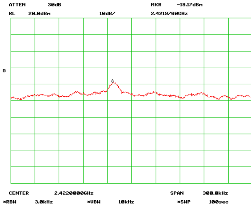
PSD - Low Channel (802.11n-40MHz)
