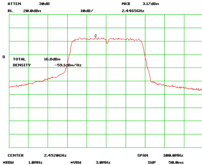
Output Power High Channel (802.11n-40MHz)
