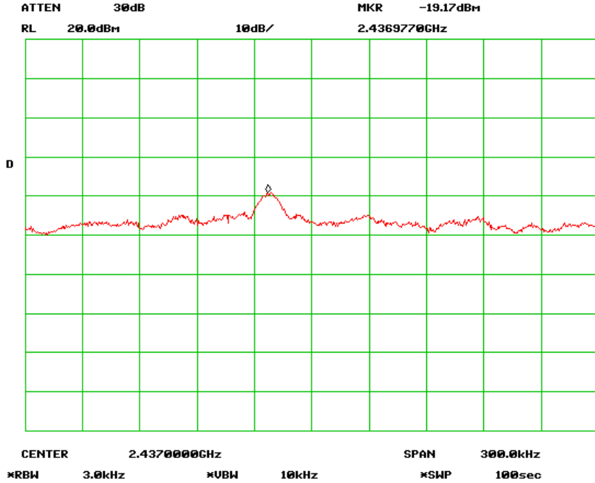
PSD - Mid Channel (802.11n-40MHz)
