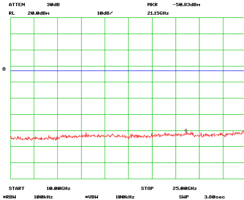
Antenna Port Emission High-4 Channel (802.11g)
