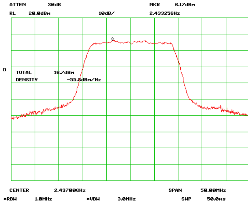
Output Power Mid Channel (802.11n-20MHz)
