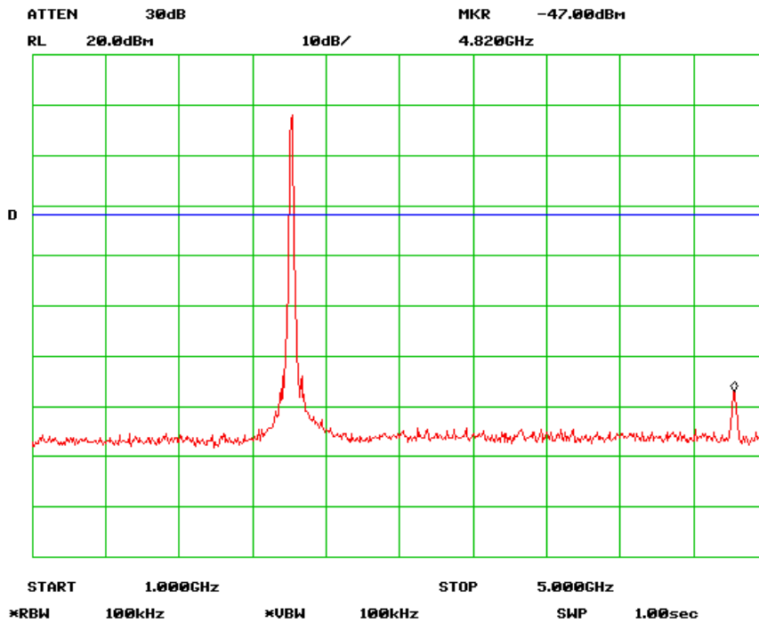
Antenna Port Emission Low-2 Channel (802.11n 20MHz)
