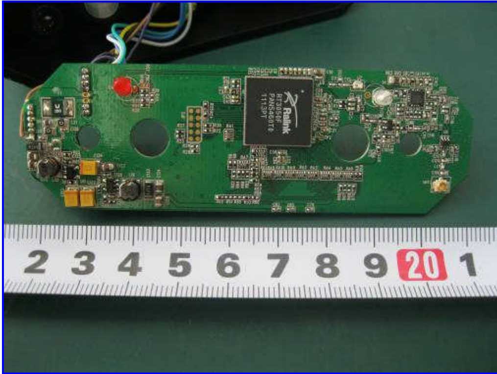
Front View of WIFI PCB Board
