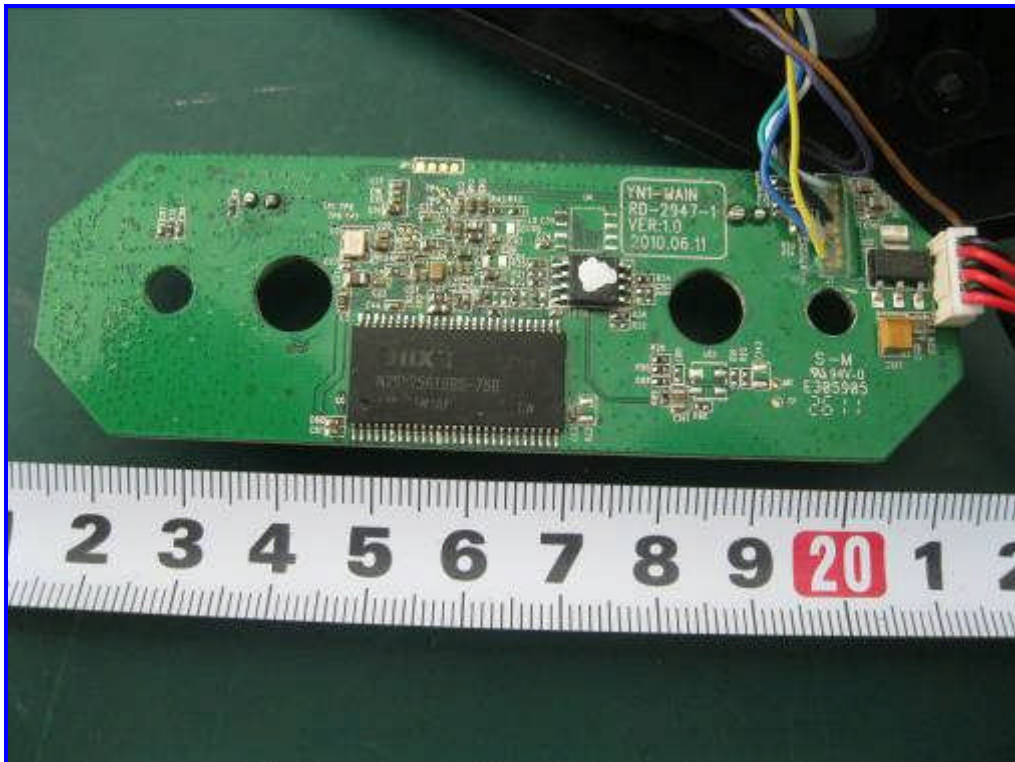
Rear View of WIFI PCB Board
