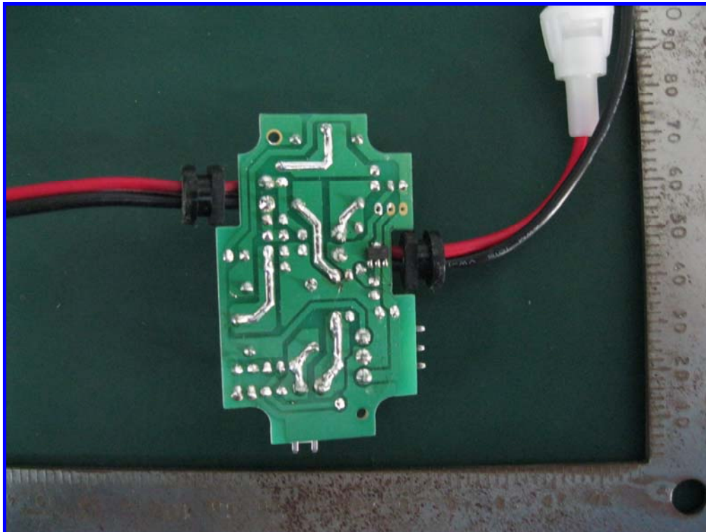
Rear View of Power PCB Board
