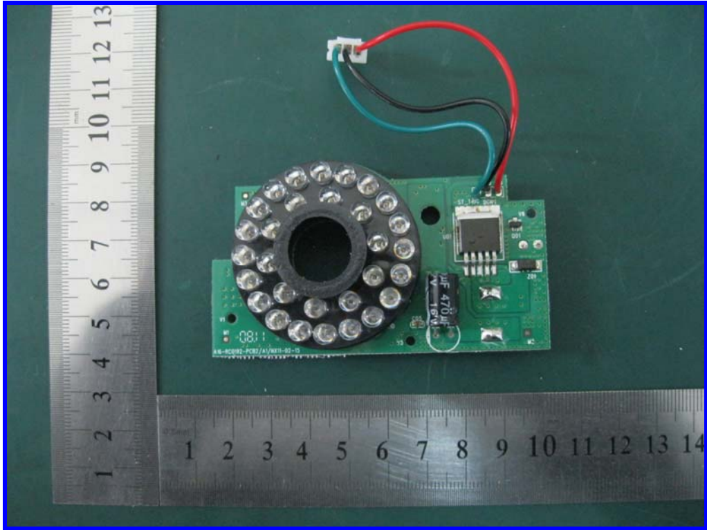
EUT-PCB Board Rear View
