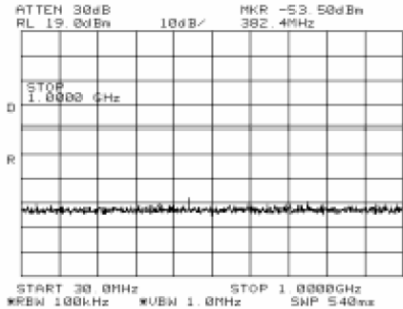
Antenna Port Emission Low Channel -1(802.11b)
