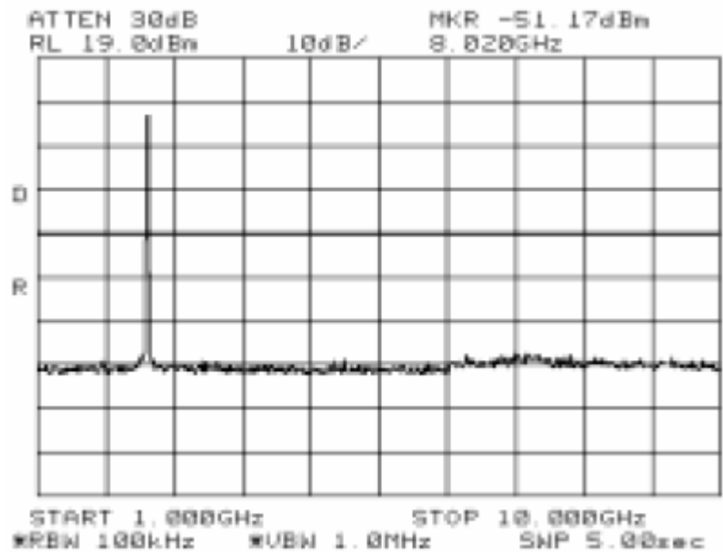
Antenna Port Emission High Channel-2 (802.11g)
