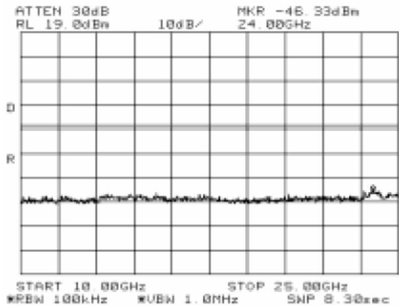
Antenna Port Emission Low Channel -3(802.11b)
