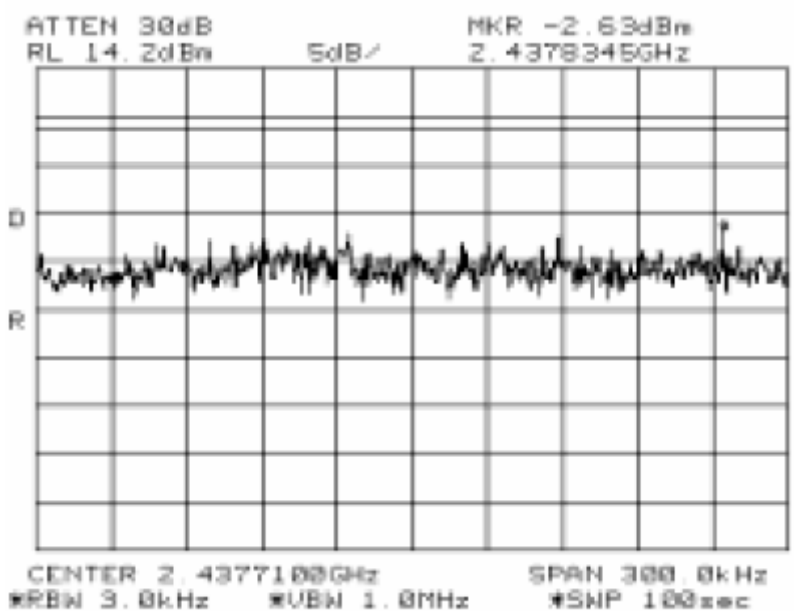
PSD - Mid Channel (802.11b)
