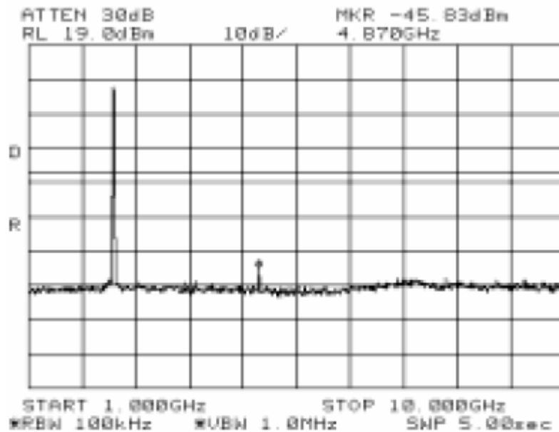
Antenna Port Emission Mid Channel-2 (802.11b)
