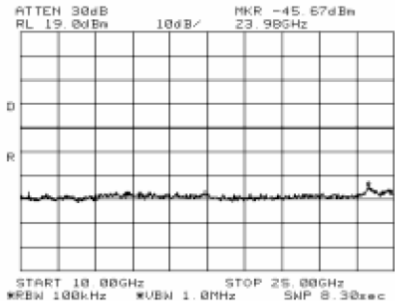
Antenna Port Emission High Channel-3 (802.11g)
