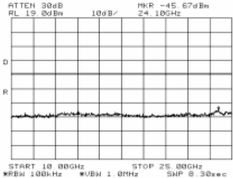
Antenna Port Emission Mid Channel-3 (802.11g)
