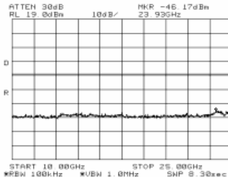
Antenna Port Emission Low Channel-3 (802.11g)
