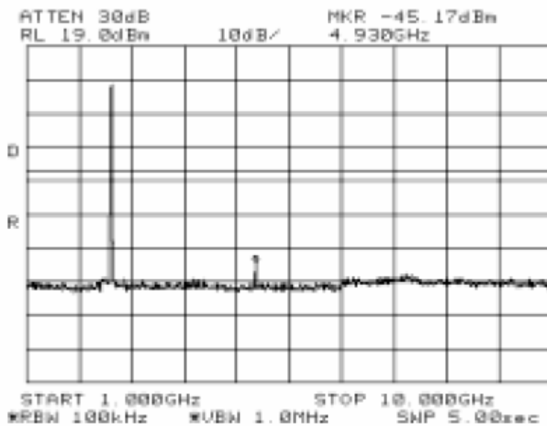
Antenna Port Emission High Channel-2 (802.11b)
