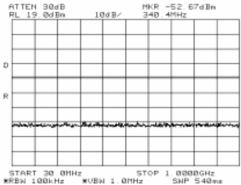
Antenna Port Emission Low Channel-1 (802.11g)
