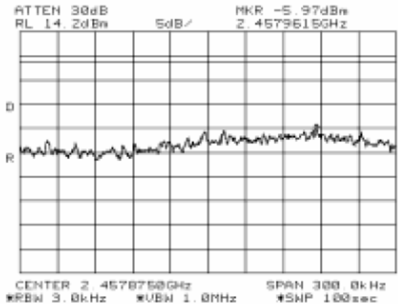
PSD - High Channel (802.11g)
