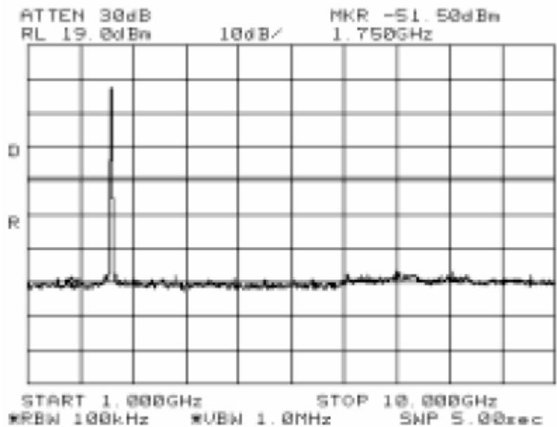
Antenna Port Emission Mid Channel-2 (802.11g)
