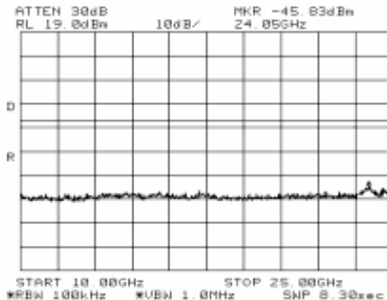
Antenna Port Emission Mid Channel-3 (802.11b)
