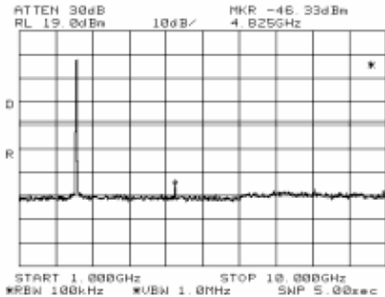
Antenna Port Emission Low Channel -2(802.11b)
