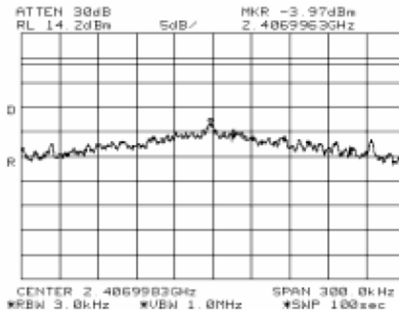
PSD - Low Channel (802.11g)
