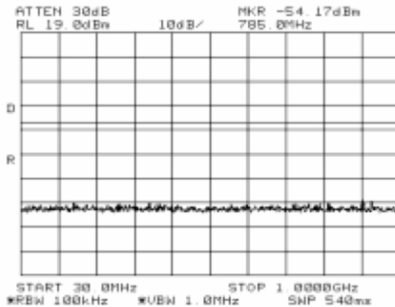
Antenna Port Emission High Channel-1 (802.11b)
