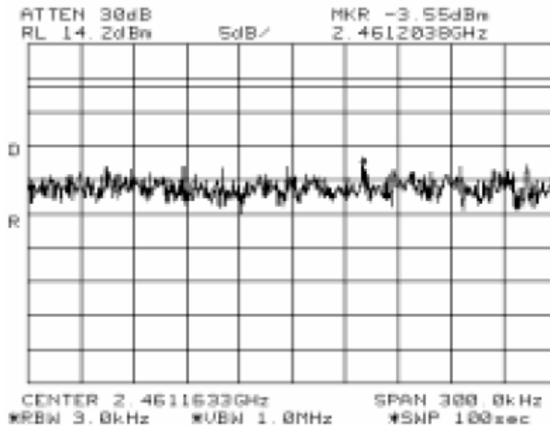
PSD - High Channel (802.11b)
