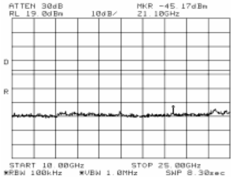
Antenna Port Emission High Channel-3 (802.11b)
