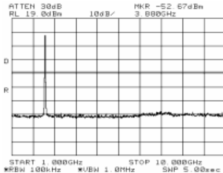
Antenna Port Emission Low Channel-2 (802.11g)
