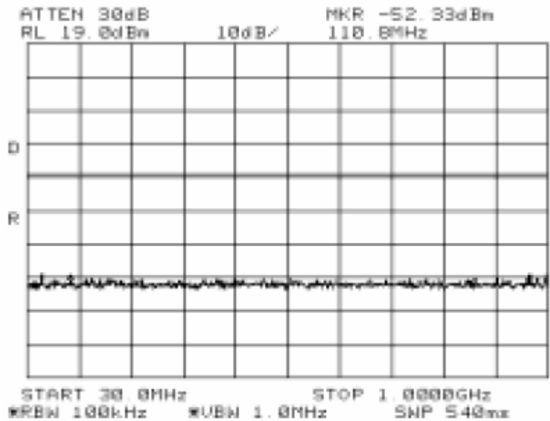
Antenna Port Emission Mid Channel-1 (802.11g)
