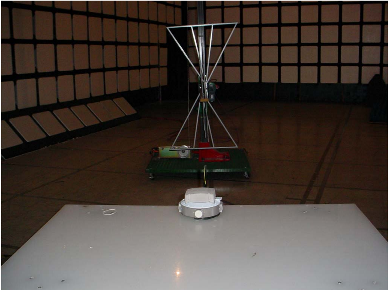
Radiated Emissions @ 3 m Test Configuration for Co-location Transmitters Radiated Emissions, Closed Enclosure
